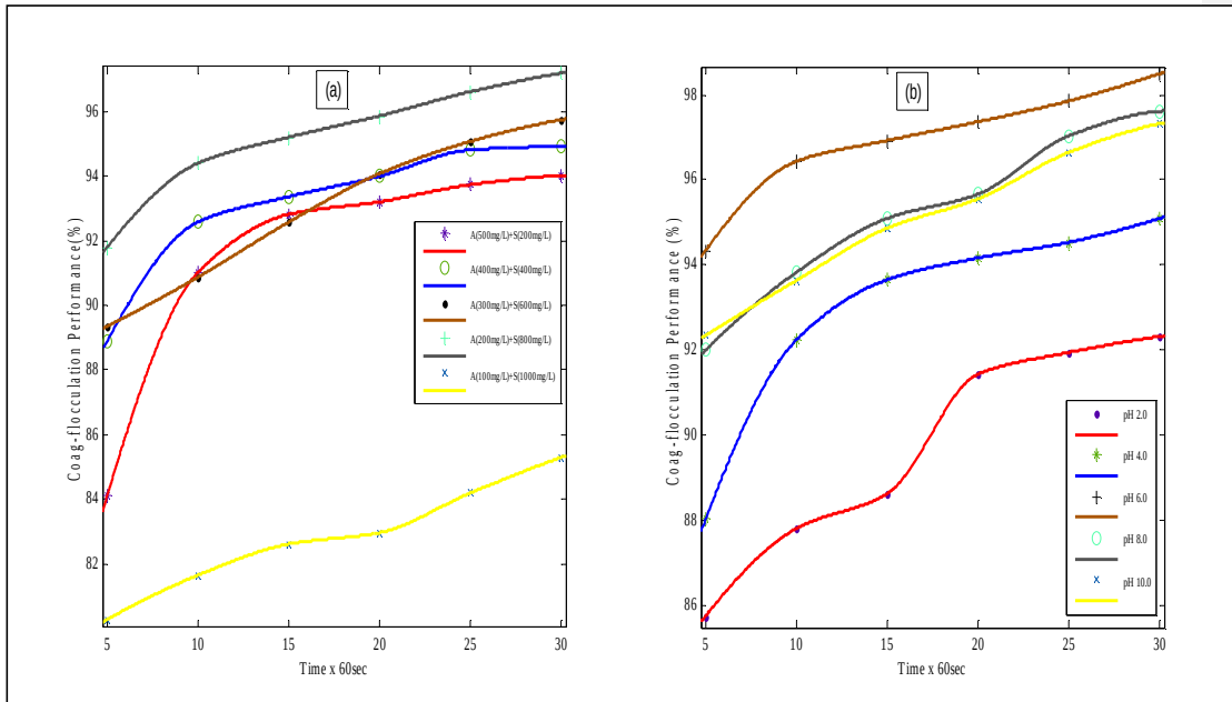
Figure 3: (a) Coag-flocculation performance as a function of time for blends of alum and SSC doses, (b) Coag-flocculation Performance as function of time for blend of 200mg/L alum and 800mg/L SSC at varying pH
