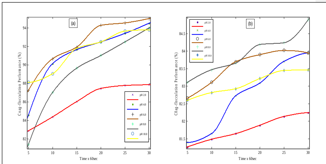
Figure 2: (a)Coag-flocculation Performance as a function of time for 200mg/L alum at varying QE pH, (b) Coag-flocculation Performance as a function of time for 600mg/L SSC at varying QE pH (what were you using)
