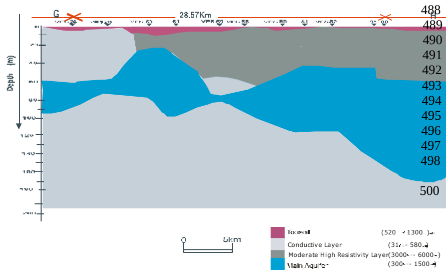
Fig.8: Interpretative IGEOelectric Cross-Section (IGCS) along profile line GH
