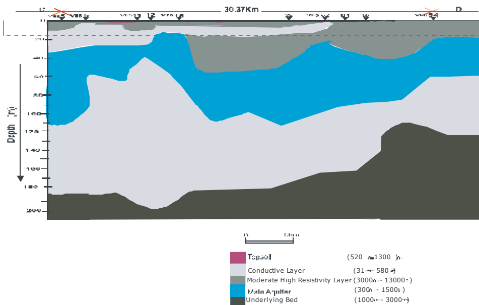
Fig.6: Interpretative Geoelectric Cross-Section (IGCS) along profile line CD
