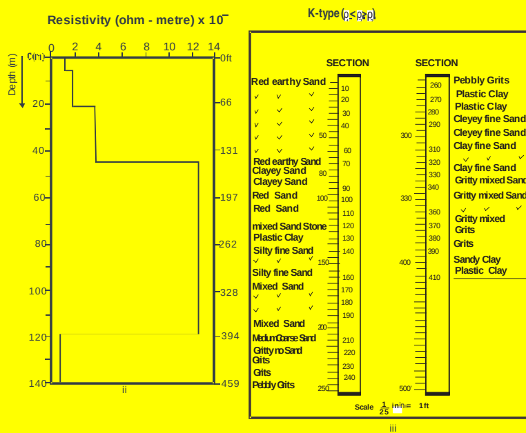
i Model curve ii Geoelectric section iii Lithology
