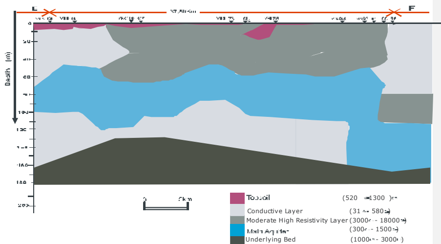
Fig.7: Interpretative Geoelectric Cross-Section (IGCS) along profile line EF
