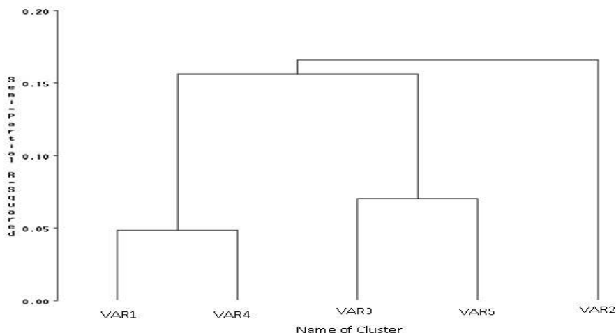
Figure 2: Dendrogram of five varieties of helmeted guinea fowl based on qualitative morphological features
