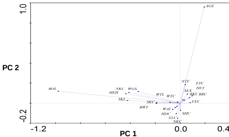
Figure 1: A biplot of the first two Principal components of helmeted guinea fowl N. meleagris in all the study zones
