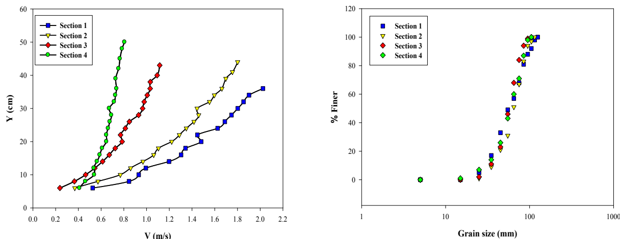
Fig. 5. (a) Velocity distributions along the pool reach (b) Particle size distributions along the pool
