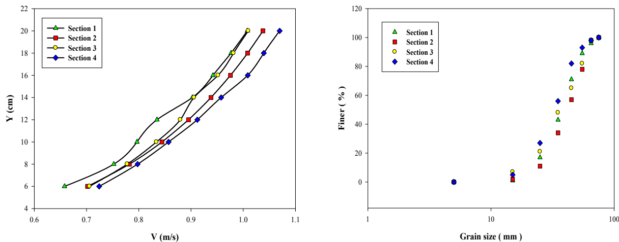
Fig. 6. (a) Velocity distributions along the plane-bed reach (b) Particle size distributions along the plane-bed
