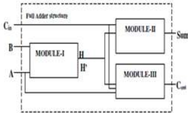
Fig.1 Block Diagram of Full Adder
