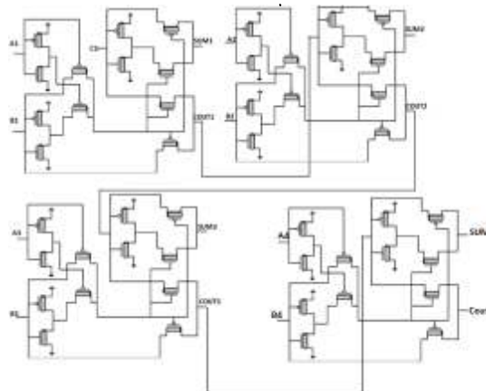
Fig. 6 Proposed 4- bit Adder
