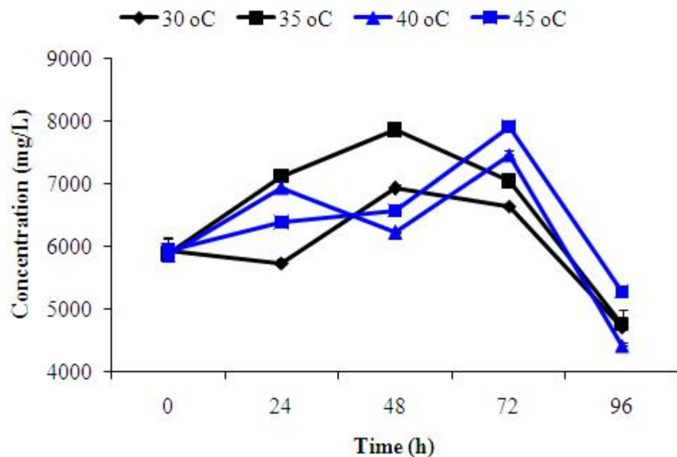
Fig. 1: Sulphate concentrations in the presence of the Aspergillus niger at the different incubation temperatures
