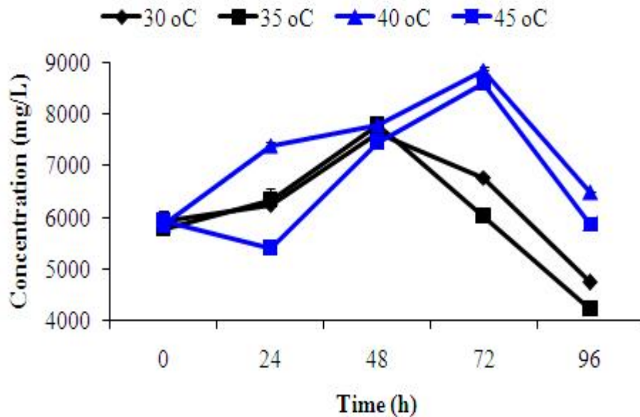
Fig. 7: Sulphate concentrations in the presence of the Staphylococcus spp. at the different incubation temperatures
