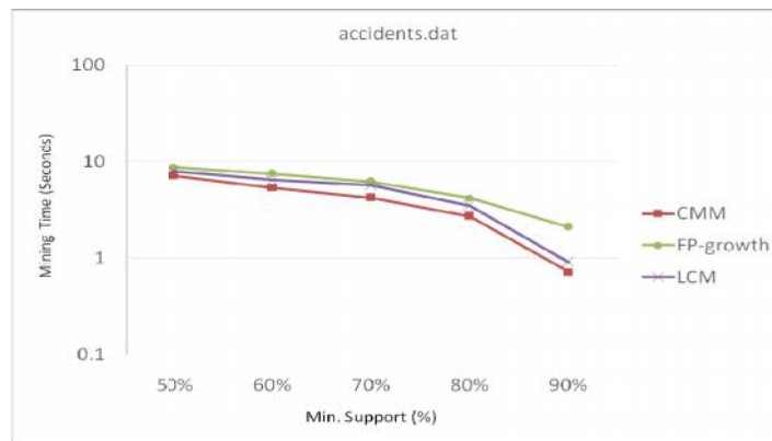
Fig. 4 Mining time for accidents dataset
