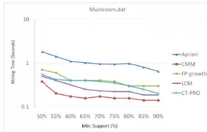
Fig. 2 Mining time for mushroom dataset
