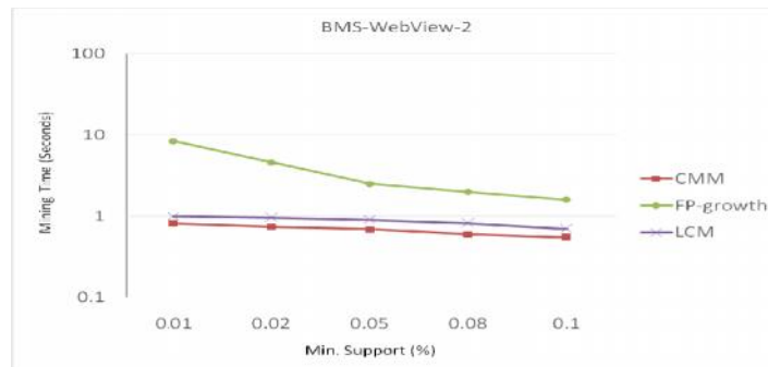
Fig. 5 Mining time for BMS-WebView-2 dataset
