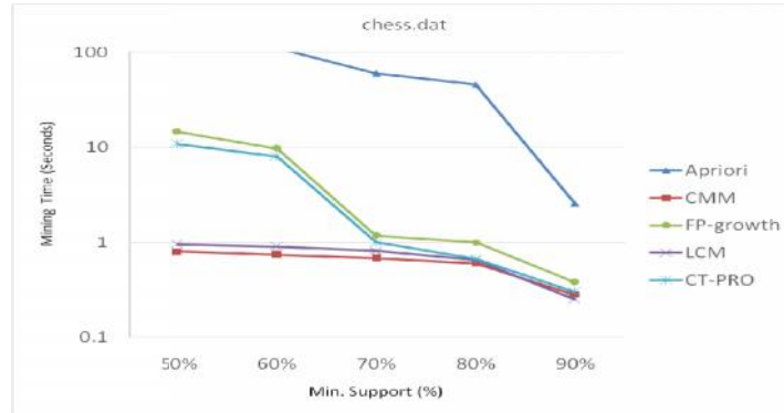
Fig. 3 Mining time for chess dataset
