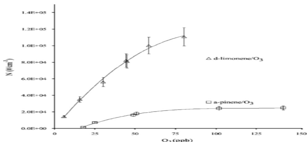
Figure 1: Effect of \text{O}_3 concentration on particle concentration
