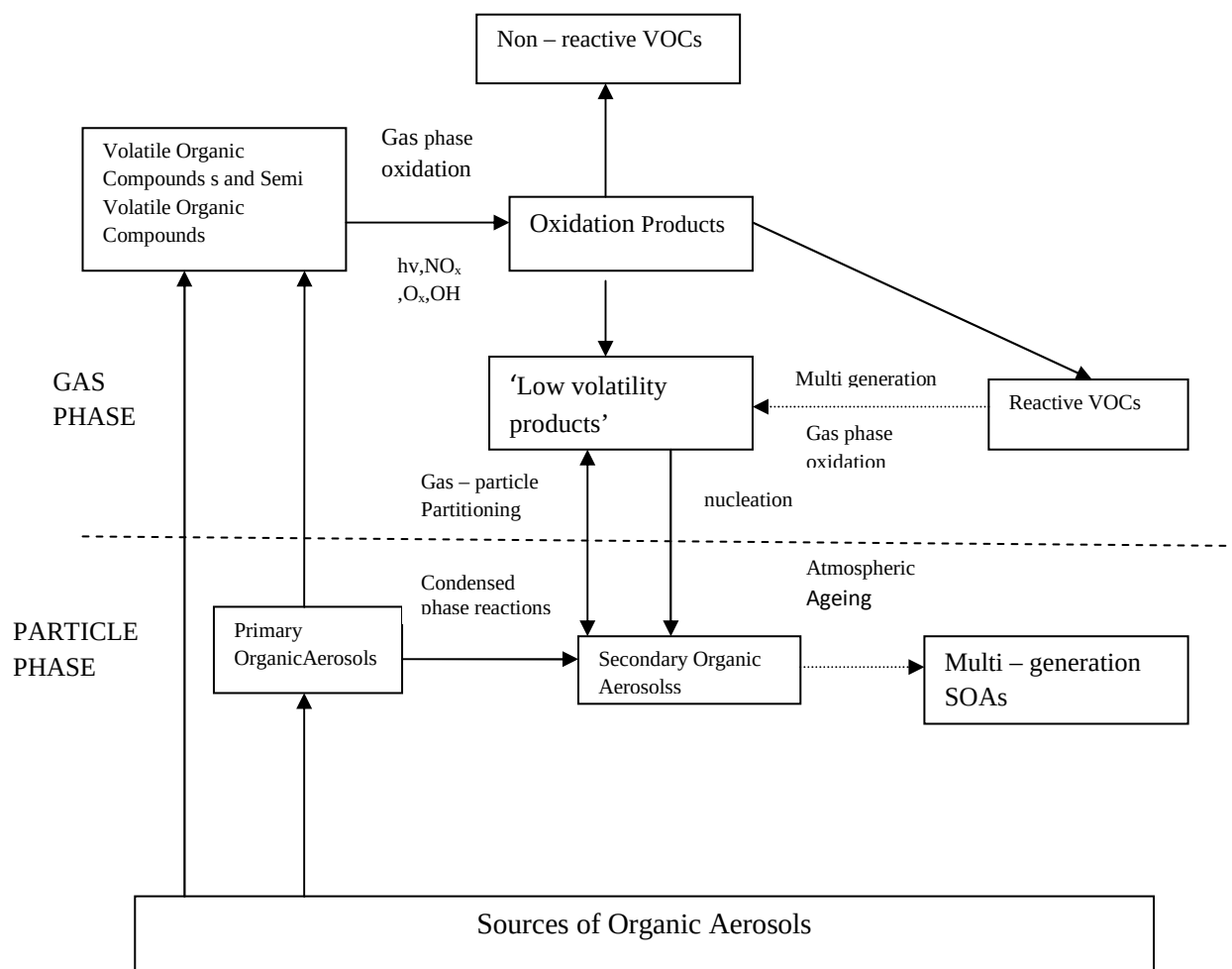
Figure 2 : Route of Formation of Secondary Organic Aerosols Source: Wang [11]
