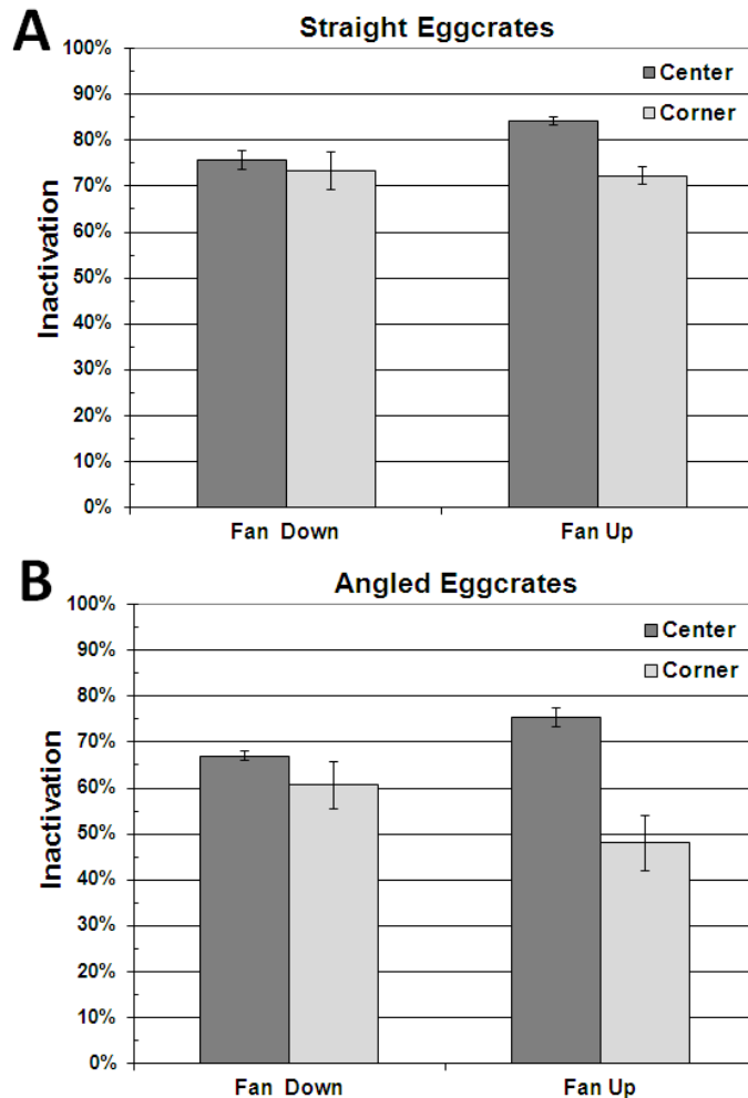
Fig. 2. Bioaerosol tests using eggcrate panels having vertical flow channels, i.e. “straight eggcrates” (A) and eggcrate panels having 45° angled flow channels, i.e. “angled eggcrates” (B). Error bars indicate standard error of the mean for independent tests.
