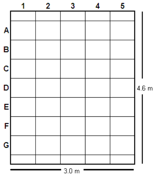
Fig. 1. Top view of schematic diagram showing the locations of 0.61-m by 0.61-m eggcrate panels in a test room with a 3.0-m high ceiling.
