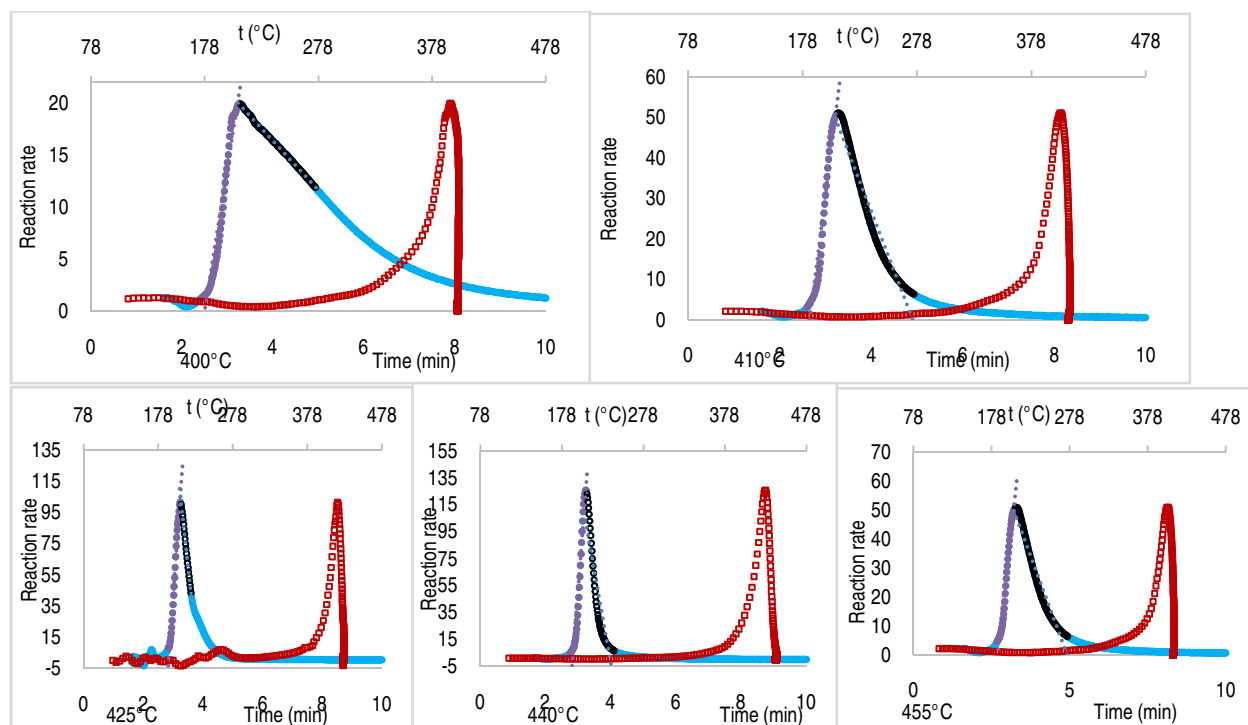
Fig 3. Variation of the initial rate of weight loss for eleven samples of PLEG at eleven thermal scans, the red color related to rate versus temperature (upper horizontal ax.) The blue color represent the rate of weight loss versus time, other colors represent the traces that were used to evaluate the values of acceleration and deceleration process.
