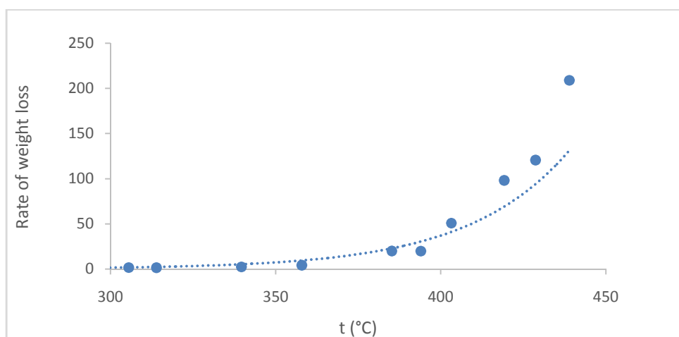
Fig 5. Variation of the values of the maximum rate of weight loss of PLEG versus temperature.
