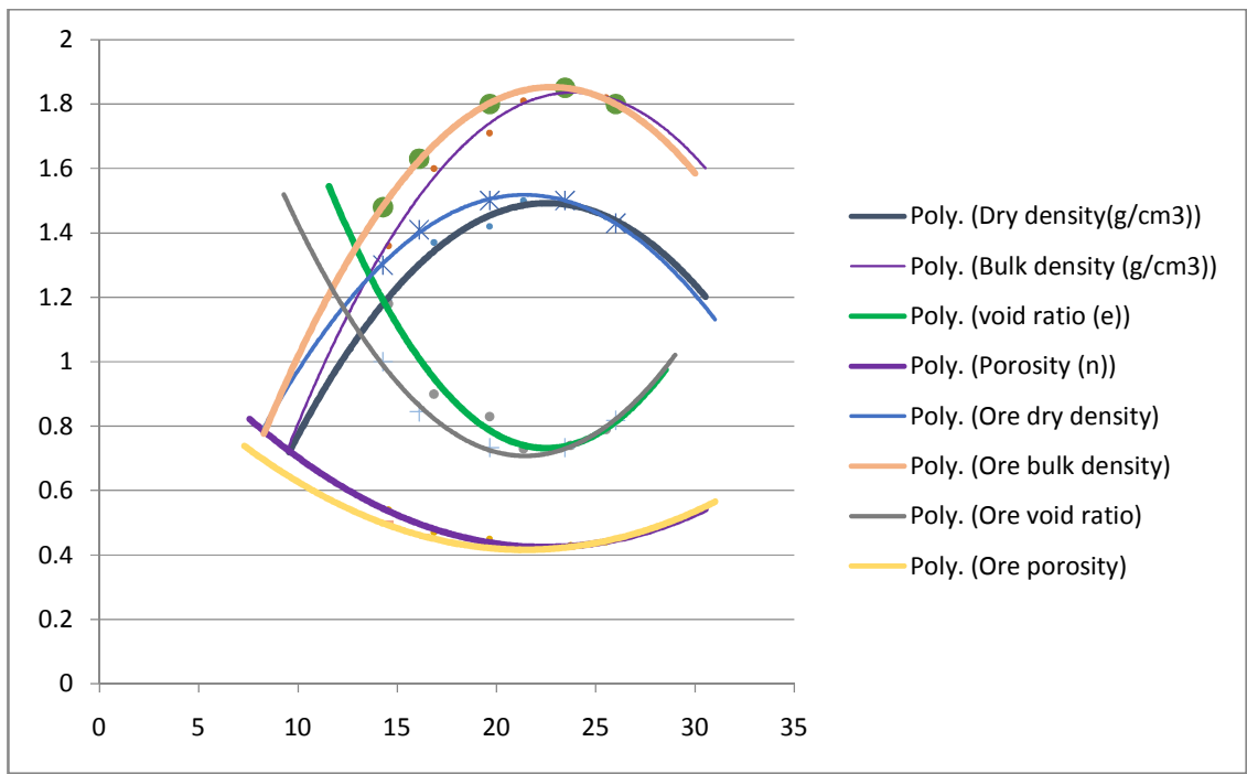
Fig.8 : Determination of various compaction indices and ratios.
