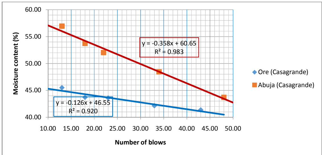
Fig. 4: Determination of LL in the sampled areas using the casagrande device
