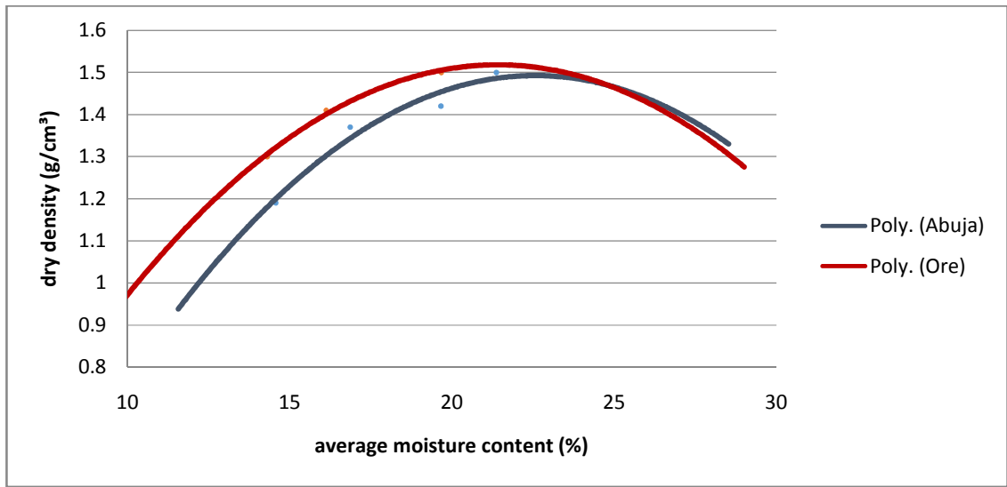
Fig.7 : Determination of maximum dry densities and optimum moisture contents
