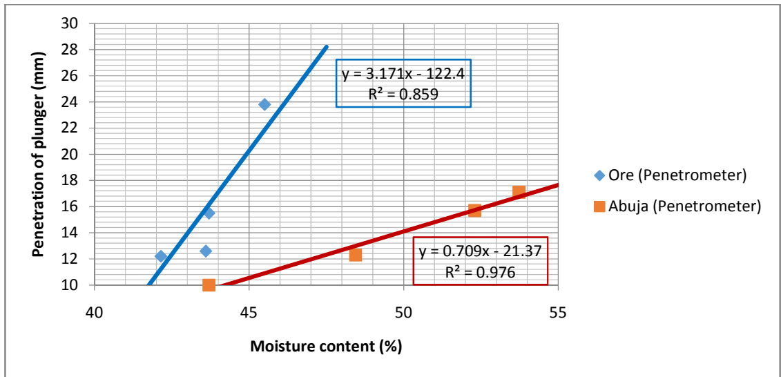
Fig. 5: Determination of LL in the sampled areas using the cone penetrometer
