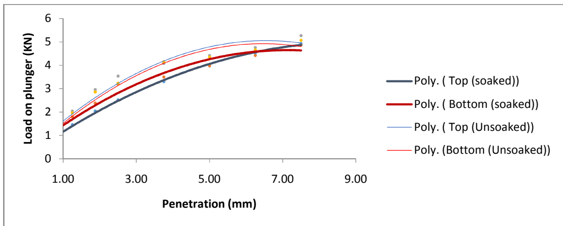
Fig. 11: CBR plots for Abs
