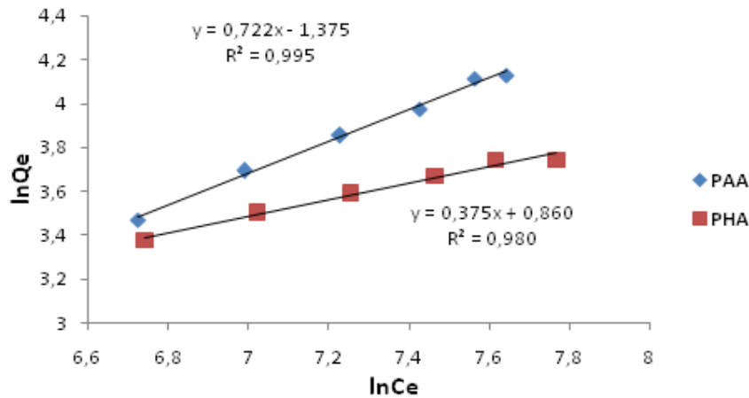
Figure 14: Linear Plot of the model of Freundlich for C_0 = 50 mg/L, V = 20 mL, pH = 4.0 , m = 0.1 g Adsorbent
