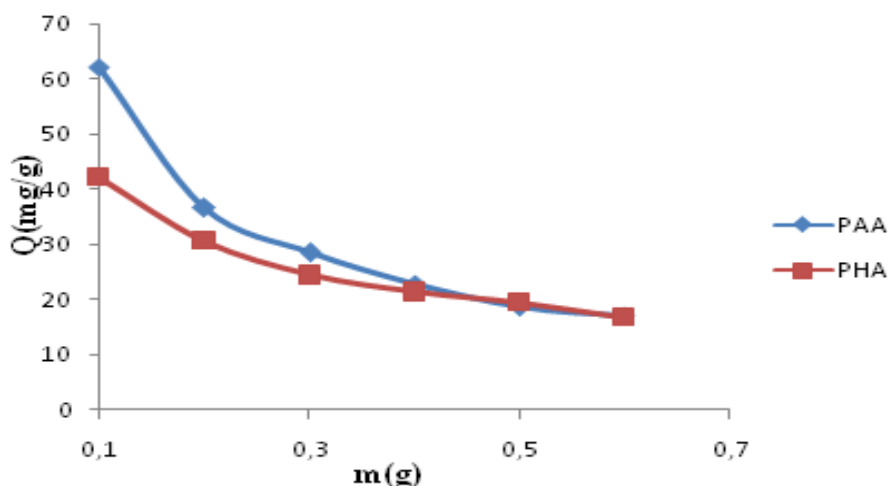
Figure 7: Influence of Absorbent dose for the Uptake of Copper (II) Ions on PAA and PHA.
