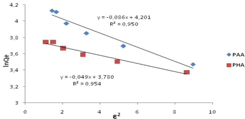
Figure 15: Linear Transform of the Model of D-K-R for C_0 = 2400 mg/L, V = 20 mL, pH = 4.0 , m = 0.1 g Adsorbent
