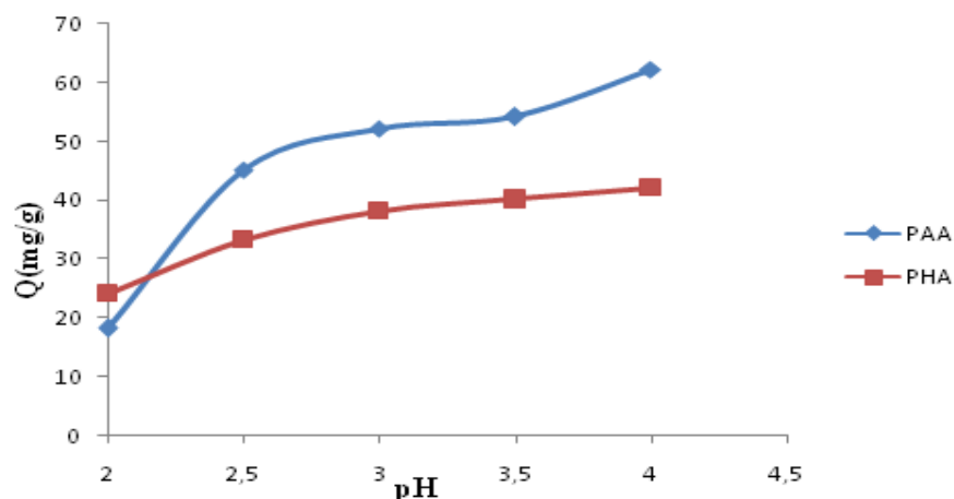
Figure 6: Influence of pH on Copper(II) ion adsorption on PAA and PHA
