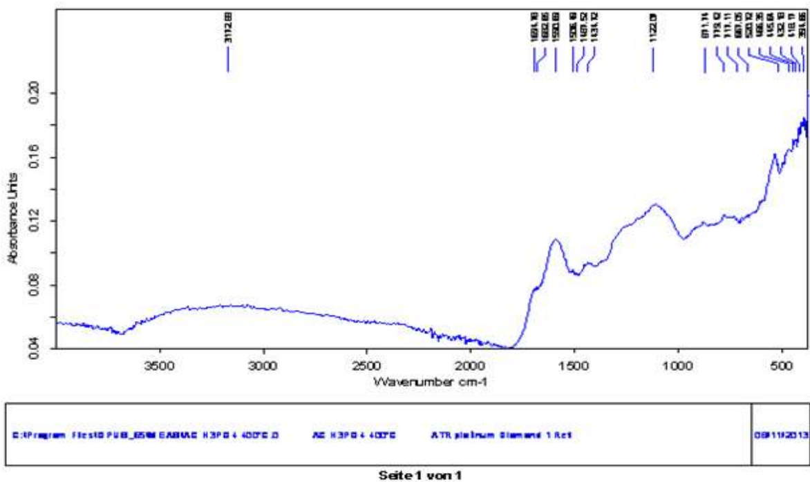
359 Figure 3: FTIR spectrum for PAA
