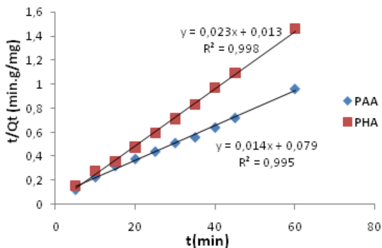
Figure 10: Linearized Pseudo-Second Order Plots for C_0=2400\text{mg/L} , V = 20 \text{ mL} , \text{pH} = 4.0 , m = 0.1 \text{ g} Adsorbent
