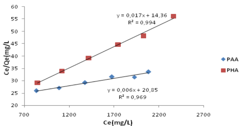
Figure 13: Linear Plot of Langmuir Model, for C_0 = 2400 mg/L, V = 20 mL, pH = 4.0 , m = 0.1 g Adsorbent
