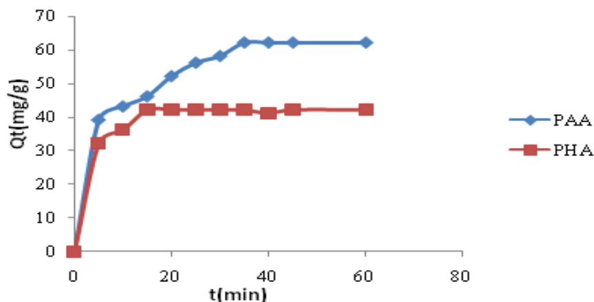
Figure 5: Effect of contact time on the adsorption of Cu(II) Ions on PAA and PHA.
