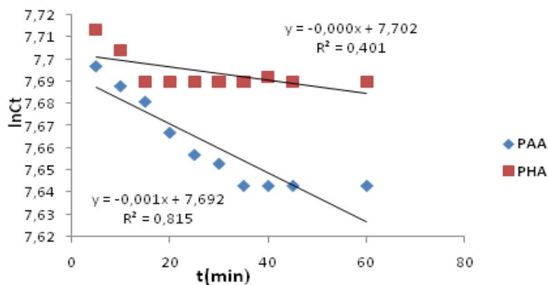
Figure 9: Linearized Pseudo-First Order Plots for C_0=2400\text{mg/L} , V=20\text{mL} , \text{pH}=4 , m=0.1\text{g} Adsorbent
