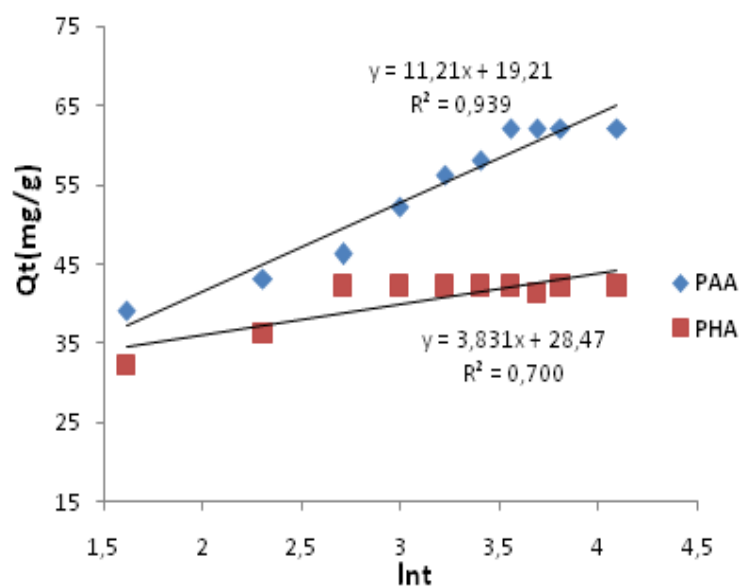
Figure 11: Linearized Elovich plots for C_0 = 2400 mg/L, V=20 mL, pH = 4.0 , m = 0.1 g Adsorbent
