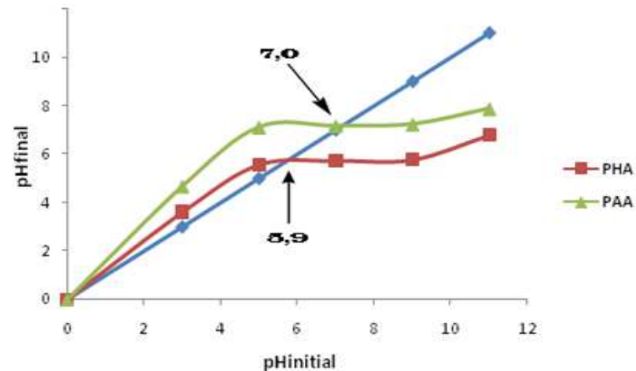
Figure 2 : Graph for the determination of \text{pH}_{\text{zpc}} for PAA and PHA.
