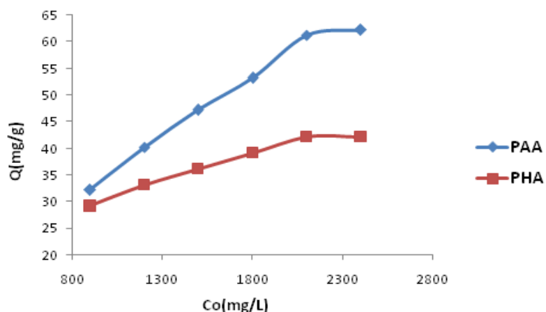
Figure 8: Effect of initial concentration on Copper (II) Ion Adsorption on PAA and PHA.
