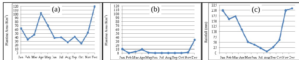
Figure 1. Planting calendar of irrigated (a) and rain-fed farm (b), in relation to rainfall pattern (c). Source: Annual report of planting area for 2012 [24].
