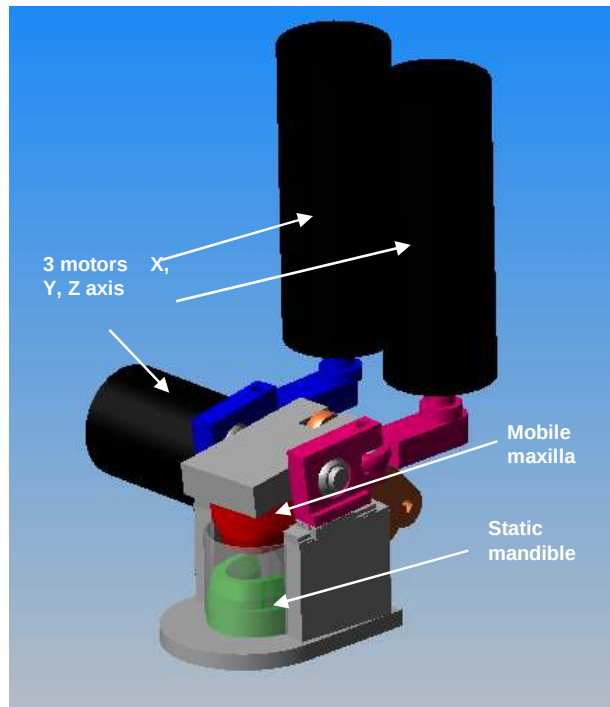
Figure 4: Simulation of the oral cavity with the chewing bench and motors
