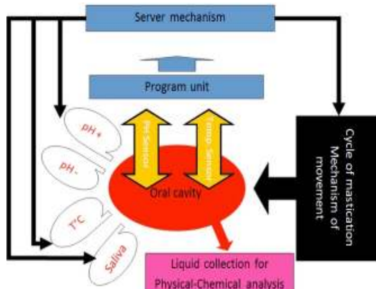
Figure 1: chewing bench principle
