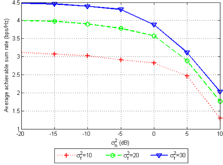
Fig. 4. Performance of the proposed algorithm for different values of \sigma_f^2
