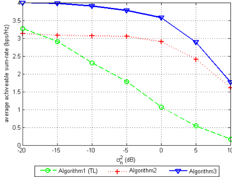
Fig. 2. Comparison of different sum rate maximization methods
