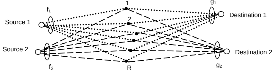
Fig. 1. A system consists of R relays and 2 source-destination pairs [10].
