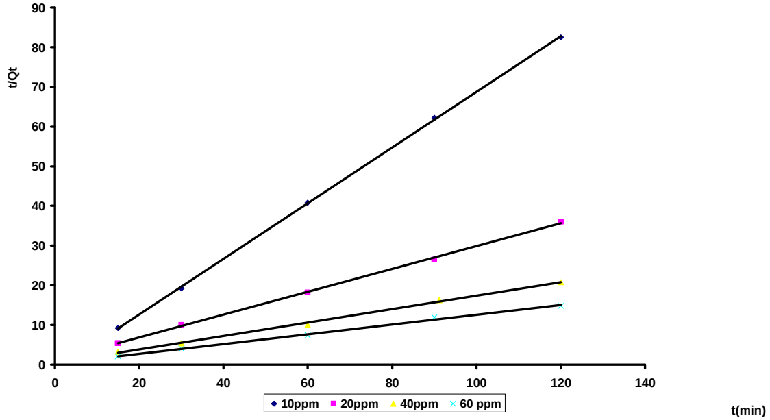
Fig.11. Pseudo-second-order kinetics for adsorption of \text{Cd}^{2+} onto clay
