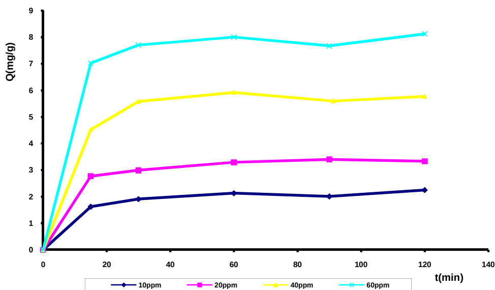
Fig.5. Effect of agitation time and initial concentration of \text{Cd}^{2+} on the adsorption of \text{Cd}^{2+} (conditions: carbon concentration, 0.2g/50 mL.)
