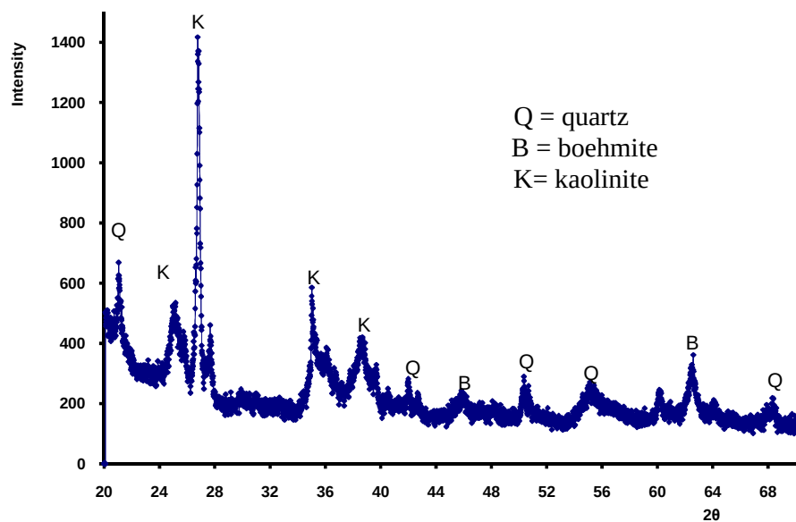
Fig.1. X-ray diffraction patterns of the natural clay.
