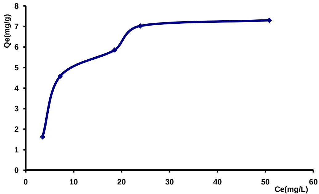
Fig. 7. Adsorption isotherms of cadmium
