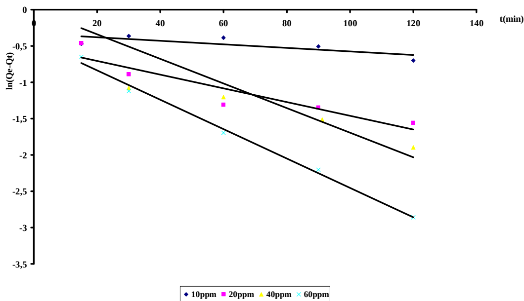
Fig.10. Pseudo-first-order kinetics for adsorption of \text{Cd}^{2+} onto clay
