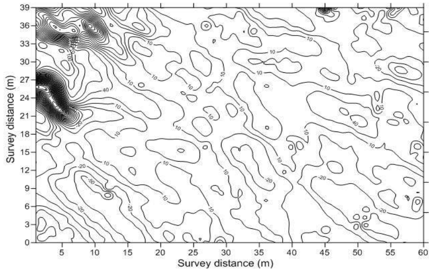
Fig. 3 Residual anomaly of Ejuona data
