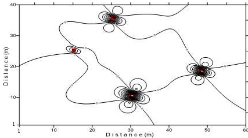
Fig. 1: Calculated magnetic anomalies superimposed on their sources
