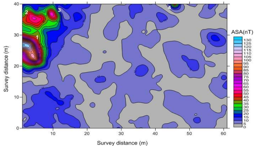
Fig. 4 Analytic signal amplitudes of Ejuona magnetic data
