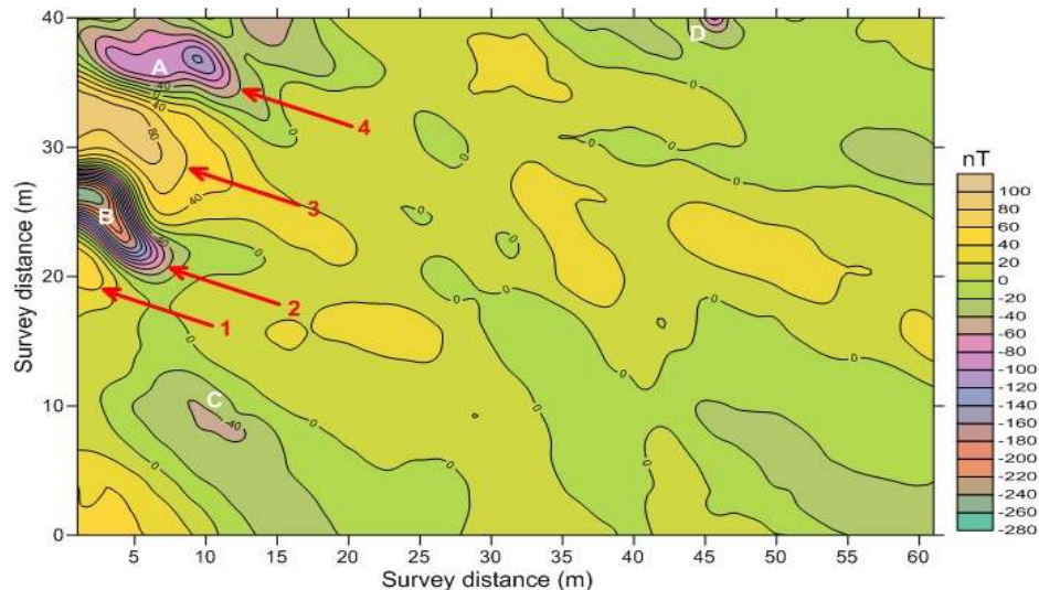
Fig. 5 Ejuona data upward continued by 0.5 metre and showing only major anomalies: A, B, C and D. (Coordinates of the origin: 7^\circ 22.75' \text{ E} , 6^\circ 42.75' \text{ N} )
