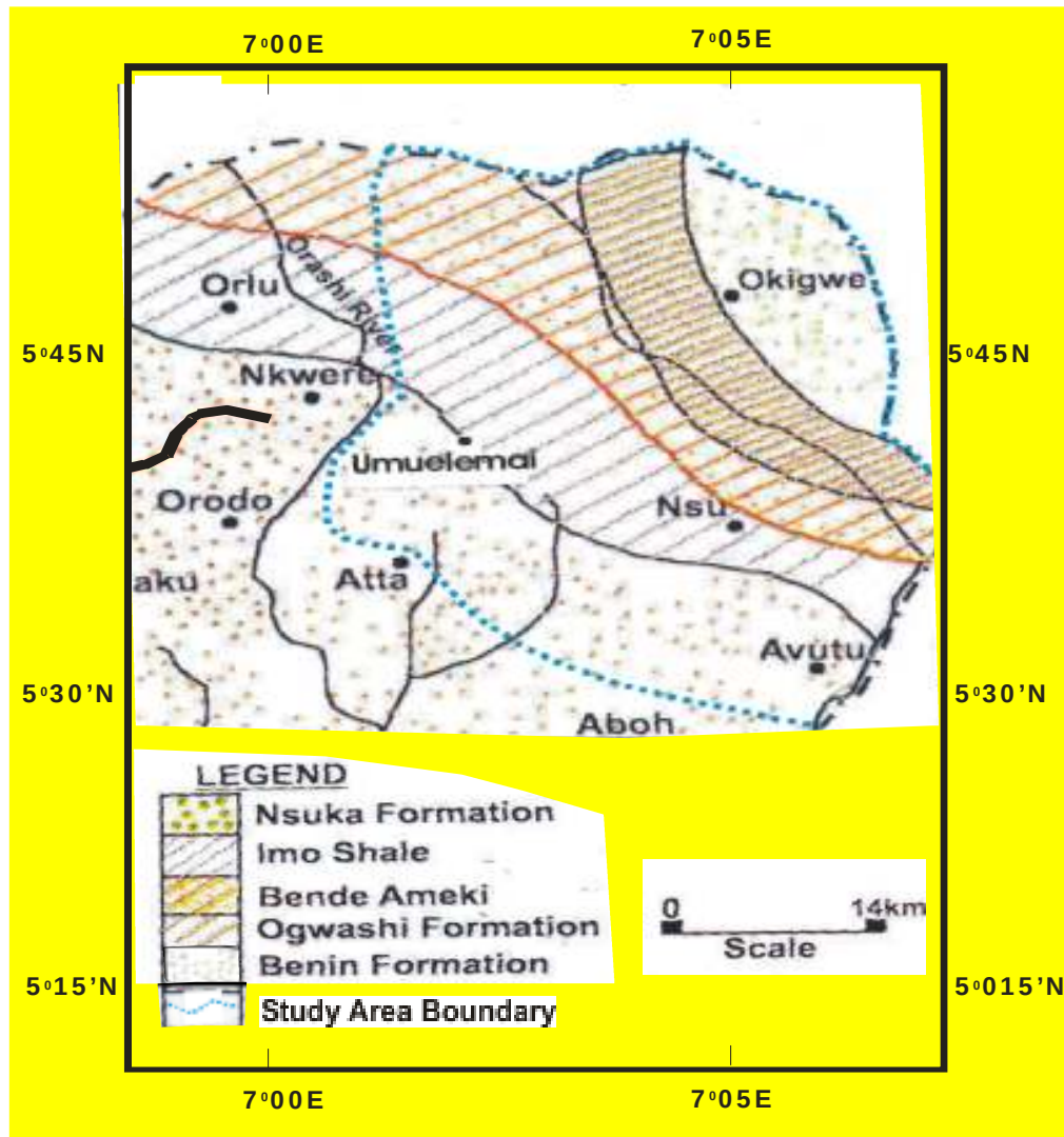
Fig. 2: Geological map of Imo State showing the study Area (Adapted from Akaolisa and Selemo, 2009).
