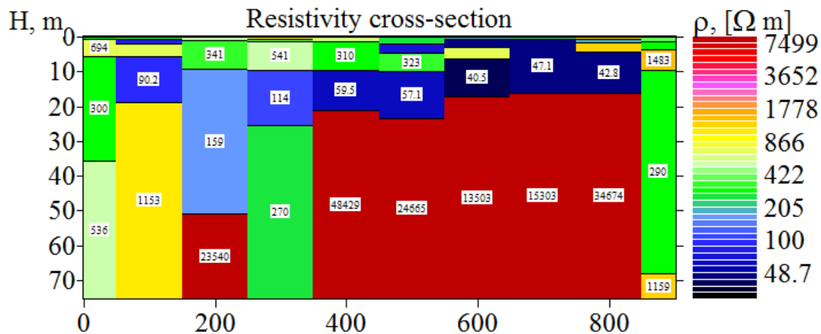
Fig.6. Resistivity cross-section for VES B 1 - B 10 .
