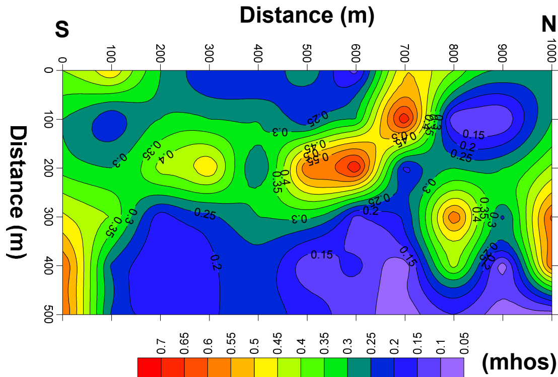
Fig. 13. Longitudinal Conductance Map
