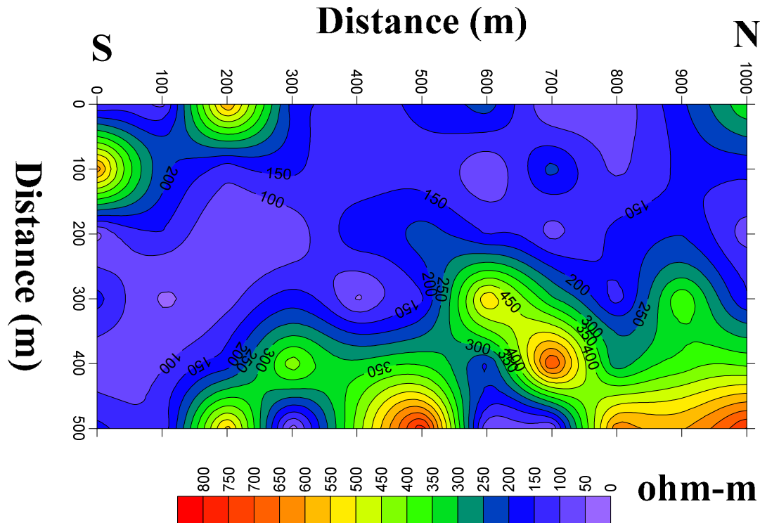
Fig.12. Weathered Basement map
