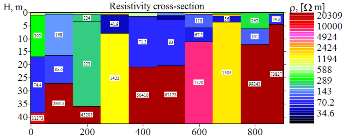
Fig.9. Resistivity cross-section for VES E_1 - E_{11}
