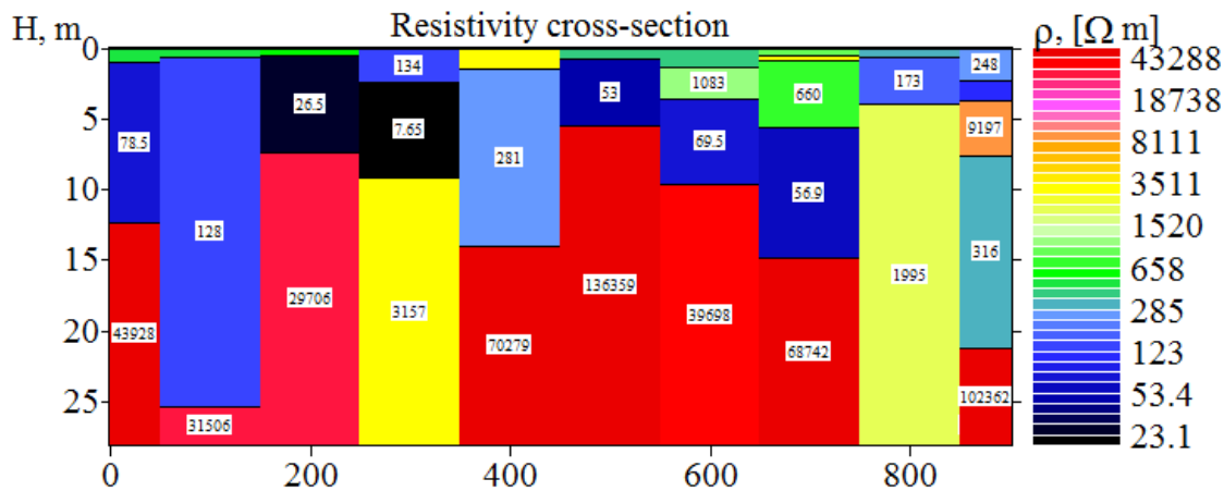
Fig.10. Resistivity cross-section for VES F_1 - F_{10}
