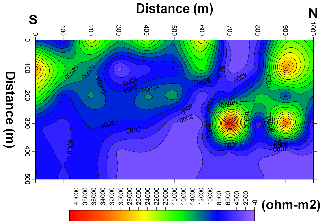
Fig. 14. Transverse resistance map
