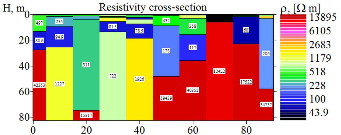
Fig.5. Resistivity cross-section for VES A_1 - A_{11} .
