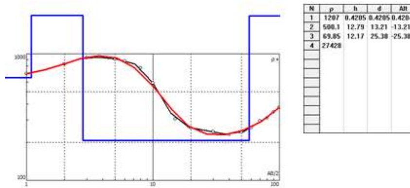
Fig. 2. Typical VES curve and model description
