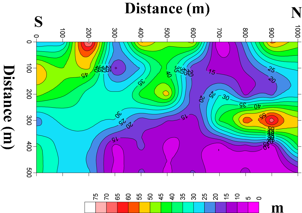
Fig 11. Isopach map of overburden
