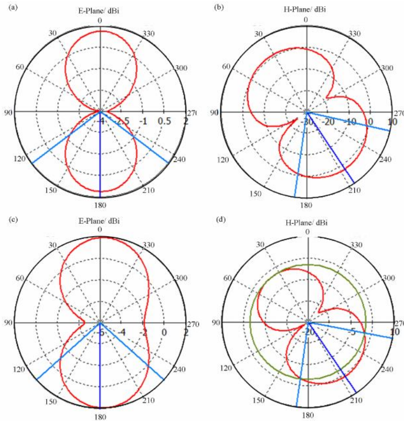
Fig. 6; Far field radiation patterns: (a) E-plane at Theta = 90° and (b) H-plane at Phi = 90° for 1.2 GHz. (c) E-plane at Theta = 90° and (D) H-plane at Phi = 90° for 1.6 GHz.
