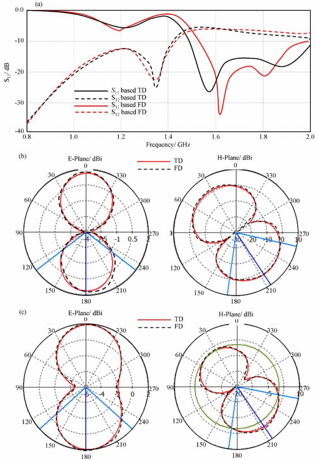
Fig. 7; Antenna performance validation using TD and FD formulations based on CST MWS 3 patches ON: (a) S_{11} , (b) Radiation patterns at 1.2 GHz, (c) Radiation Patterns at 1.6 GHz.
