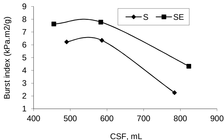
279 Fig. 4. Effect of pulp freeness on the burst index of soda (S) and soda-ethanol (SE) 280 handsheets 281 282
