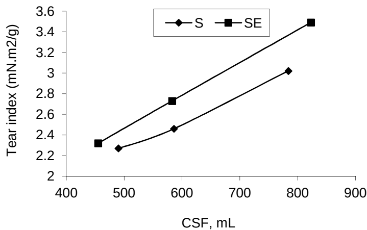
275 Fig. 3. Effect of pulp freeness on the tear index of soda (S) and soda-ethanol (SE) 276 handsheets 277 278
