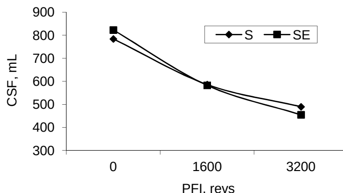
204 Fig. 1. Effect of PFI revolution on the freeness of soda (S) and soda-ethanol (SE) pulp
