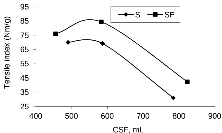
Fig. 5. Effect of pulp freeness on the tensile index of soda (S) and soda-ethanol (SE) handsheets
