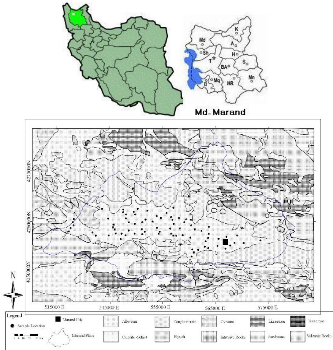
Fig. 1. Location and Geological map of the studied area [9] and Sampling locations
