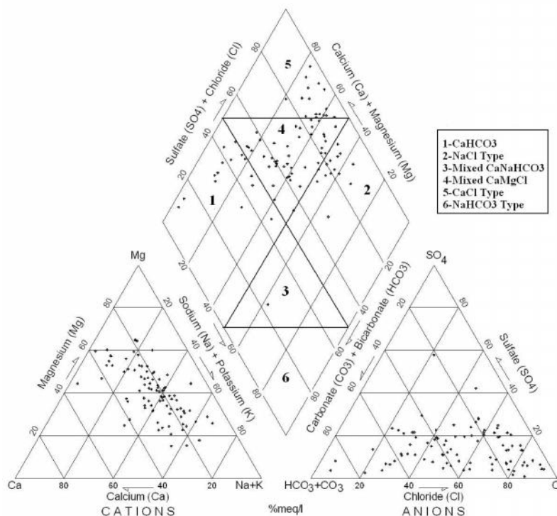
Fig. 2. Piper diagram showing hydricchemical facies of groundwater
