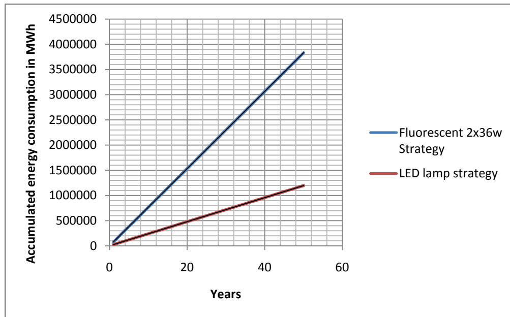
619 620 Fig. 1: predicted saving energy during 50 years is equal to 2,635.64 GWh. 621 622 623
