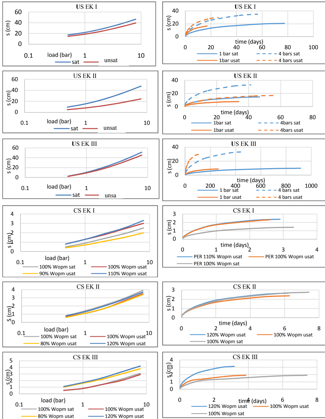
Fig. 4. Settlement (s) diagrams as function of load (a), and of time (b).
