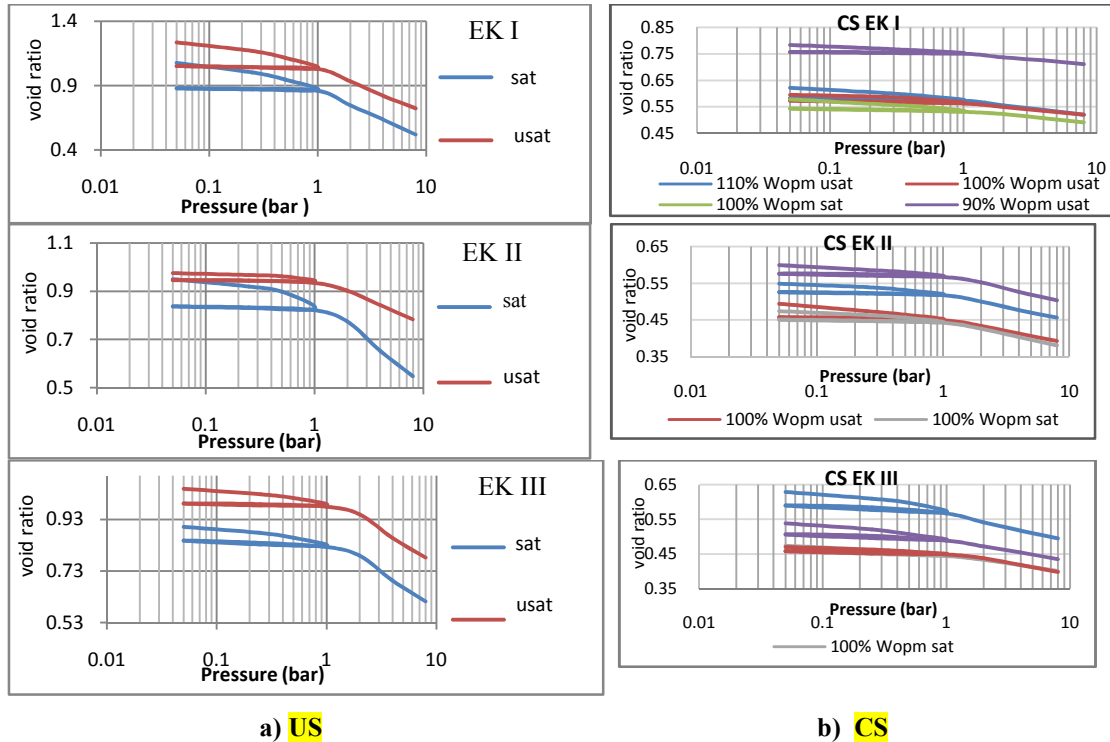
Fig. 3. curves of compressibility for (a) US and (b) CS
