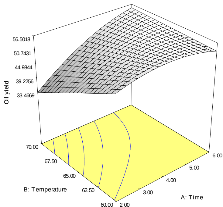
Fig.3: 3D response surface plots showing effect of temperature, time and their interactive effect on oil yield for n-hexane
