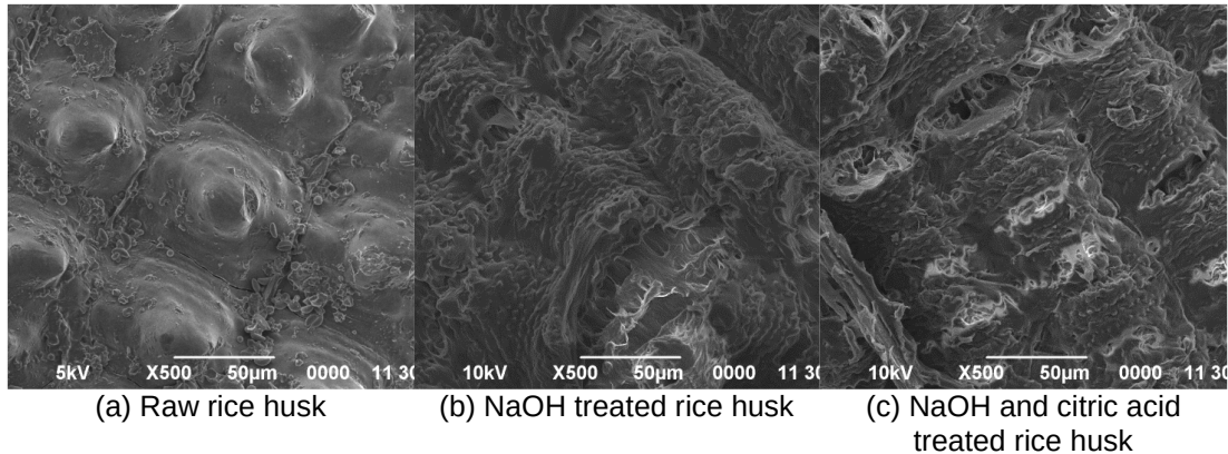
191 Figure 4. SEM images of raw and treated rice husk
