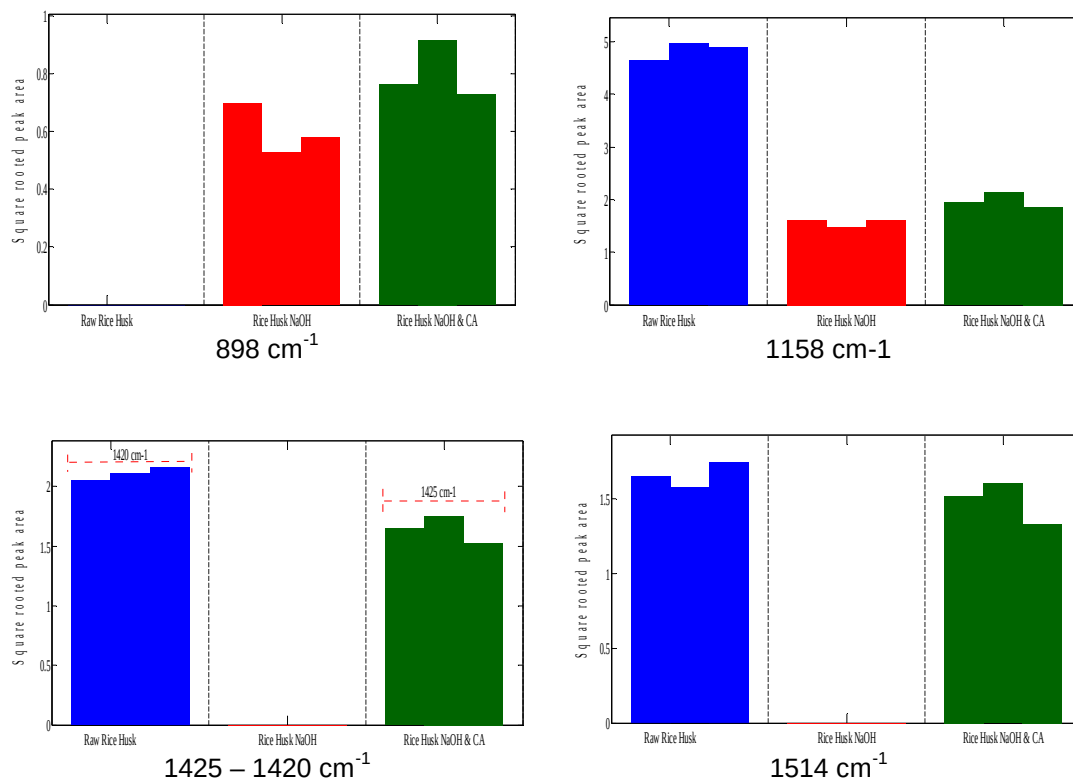
179 Figure 3: The relative abundance of some absorption bands before and after 180 treatment 181 182
