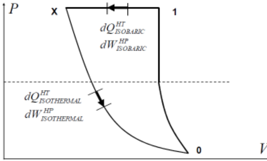
Figure 2 – Isobaric-Isothermal process (1-X-0) connecting any two states
