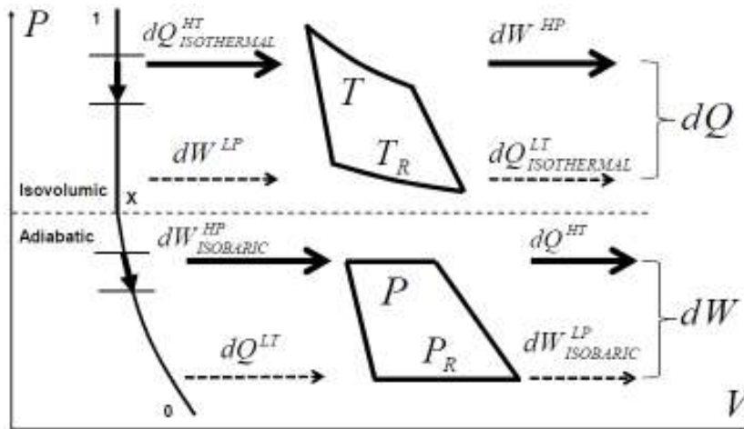
Figure 1 – Isovolumic-Adiabatic process (1-X-0) connecting any two states
