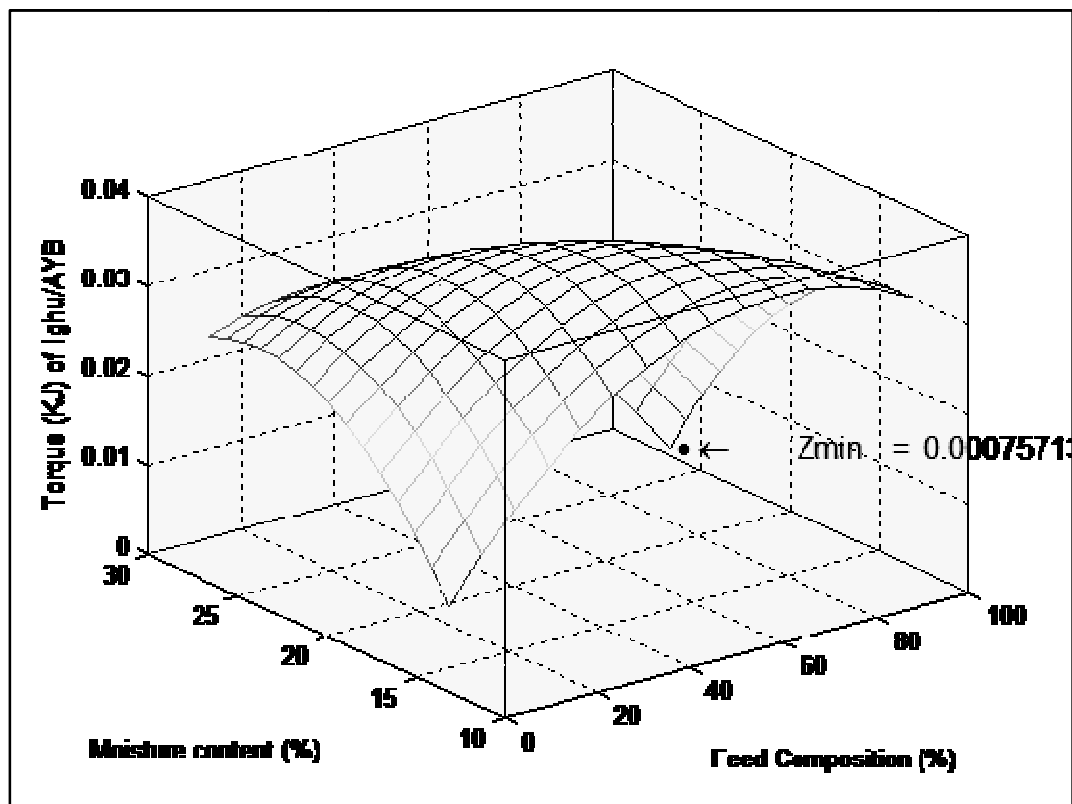
Fig 1: Effect of Moisture content and Feed composition on the Torque of extruded lghu /AYB blends.
