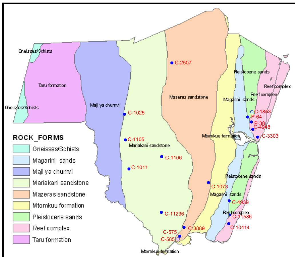
60 Figure 2: Map showing the NNE-SSW trending geological formations and study boreholes of 61 Kilifi County (adapted from the geological map of Kenya)
