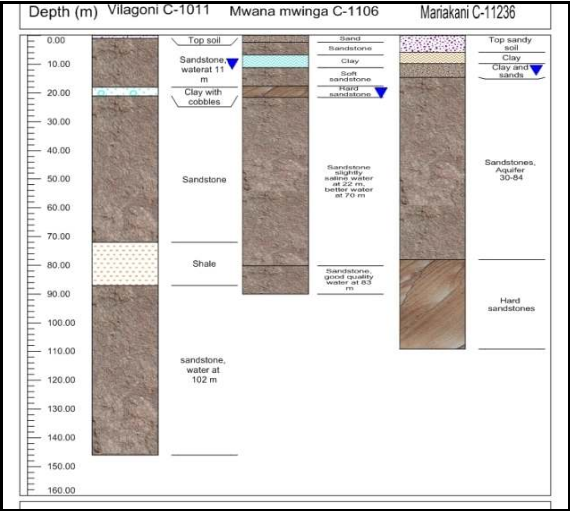
Figure 7: Subsurface information for boreholes drilled into Mariakani Sandstones
