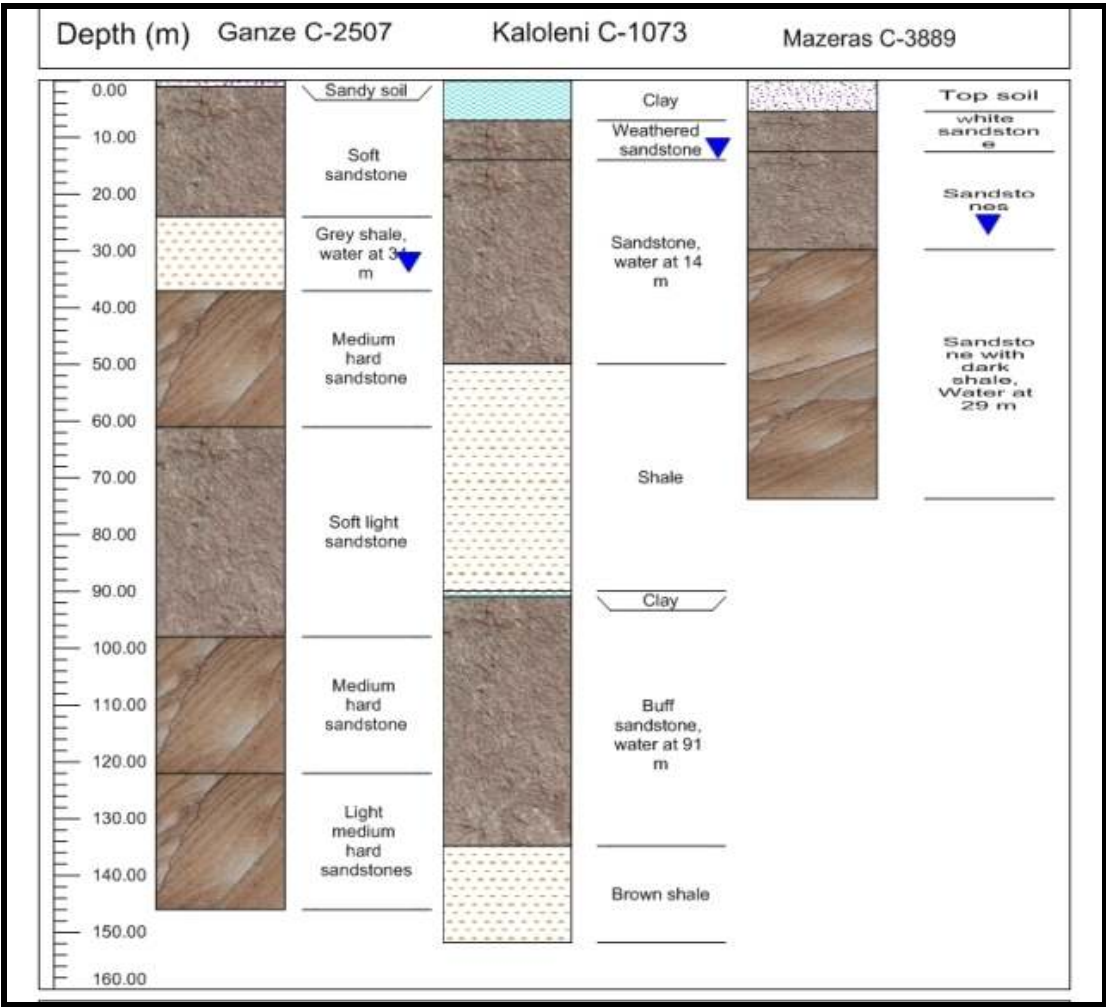
207 208 Figure 6: Subsurface information for boreholes drilled into Mazeras Formation 209
