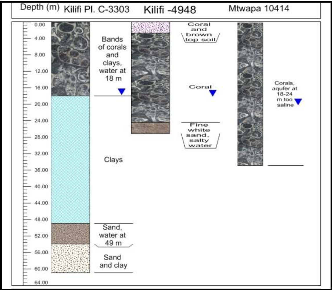
168 169 Figure 4: Subsurface information for boreholes drilled in the vicinity of the Reef Complex
