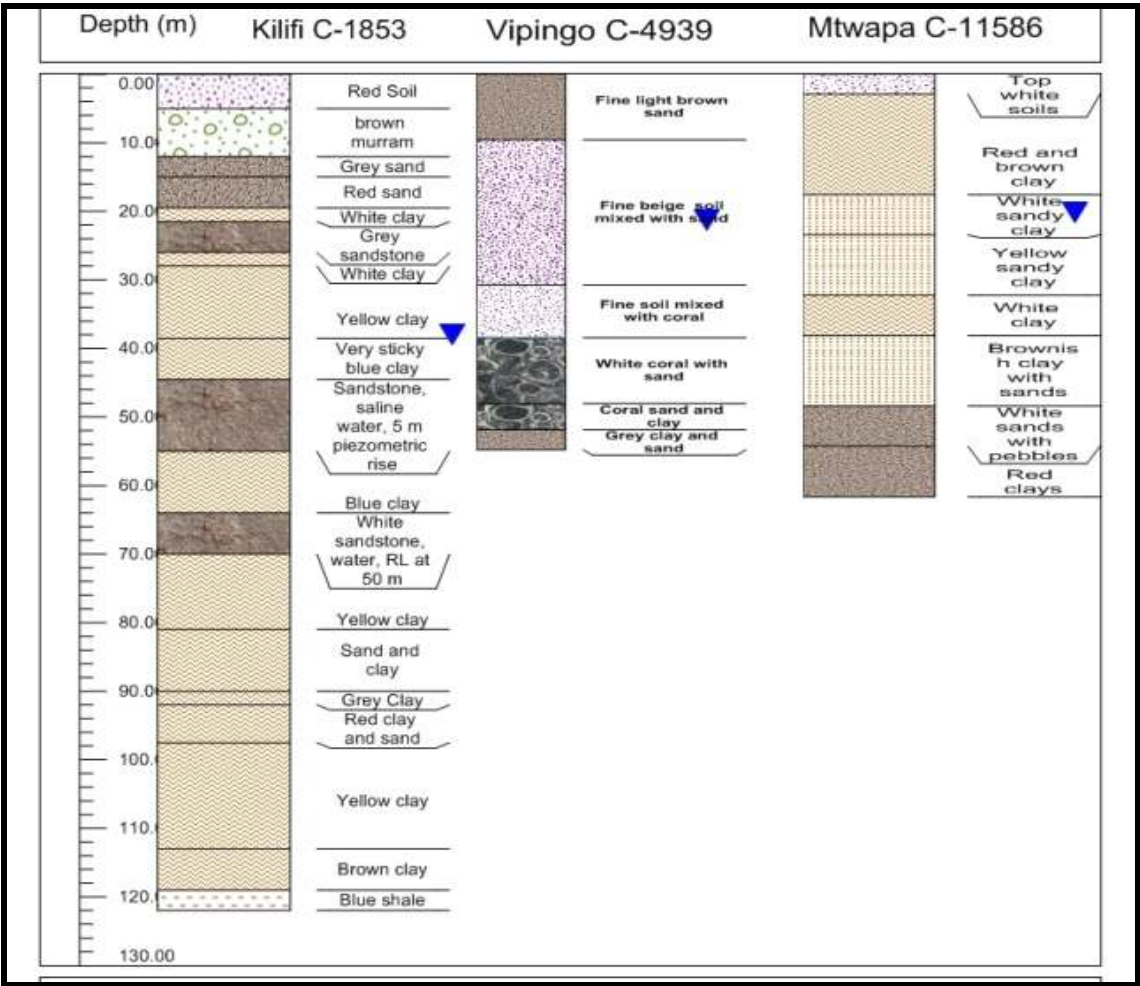
185 186 Figure 5: Subsurface information for boreholes drilled into Pleistocene and Magarini sands
