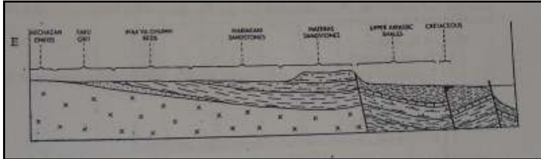
Figure 3: Schematic section through the coastlands as they are seen at the present day (After Caswell, 1953)
