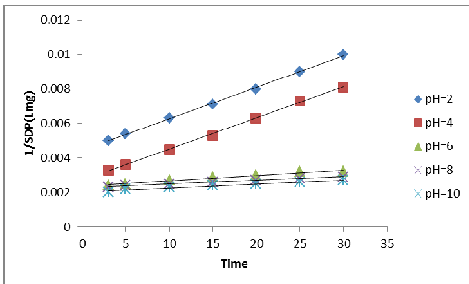
Figure 8: Representative kinetic plot of 1/\text{SDP} as a function of time for 100 \text{ mg L}^{-1} Okra dosage
