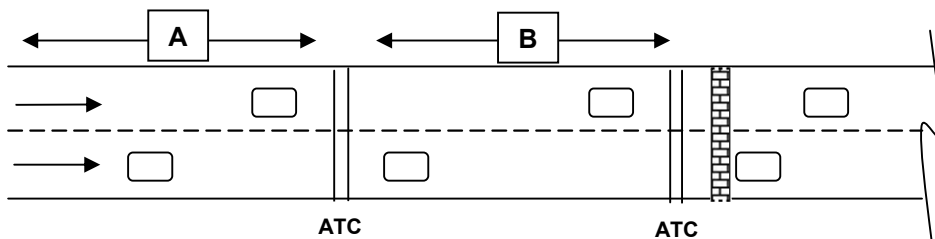
Figure 2 Typical layout of impact study site
