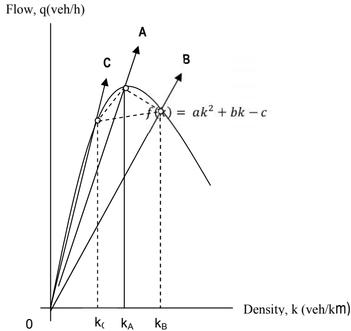
Figure 1 Flow-density curve with kinematic wave ABC
