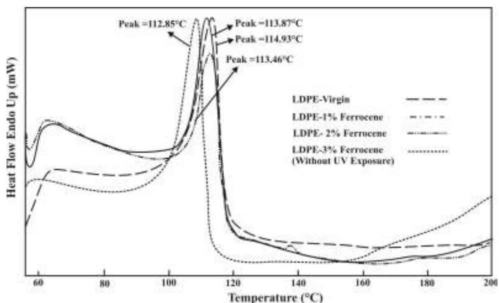
Figure 4: DSC thermogram for LDPE-1 to 3 % Ferrocene before exposure to UV radiation
