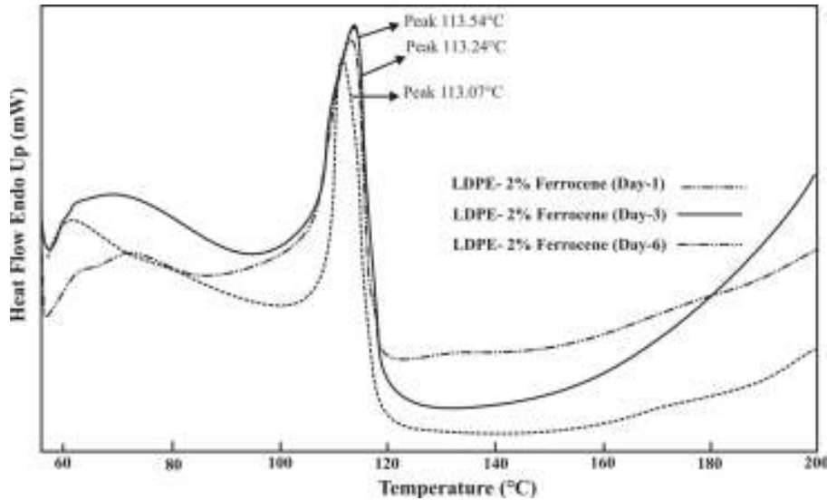
Figure .6: DSC thermogram for LDPE-2% Ferrocene after exposure to UV radiation
