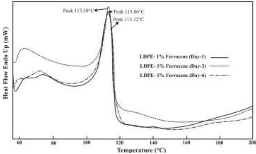
Figure 5: DSC thermogram for LDPE-1 % Ferrocene after exposure to UV radiation
