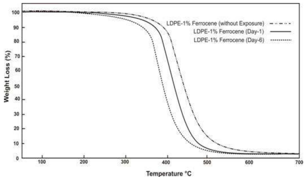
Figure.9: TGA thermogram for LDPE-1% Ferrocene after UV exposure 1 to 6 days
