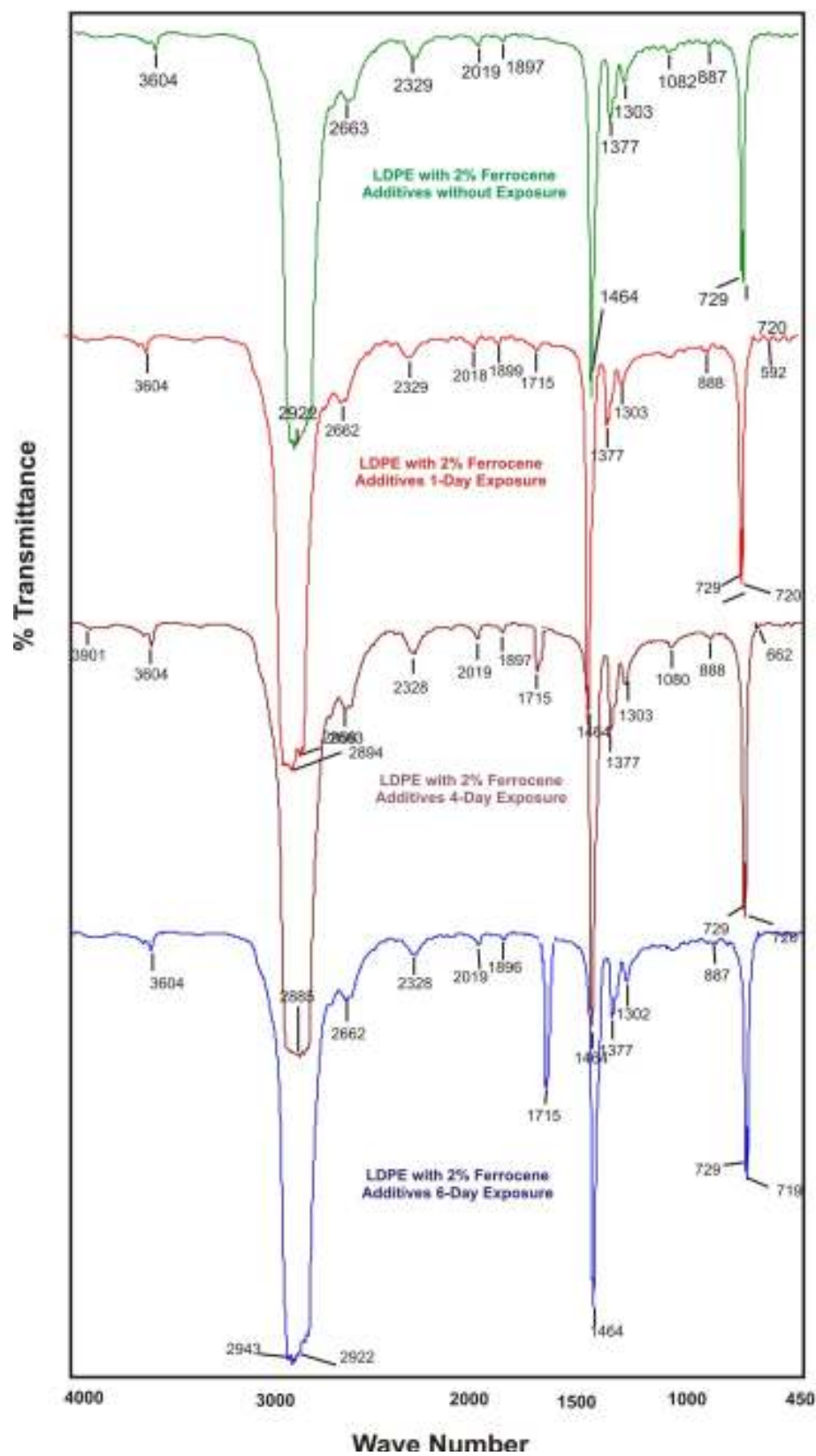
Figure.15: FTIR spectra for LDPE-2% Ferrocene after exposure to UV radiation
