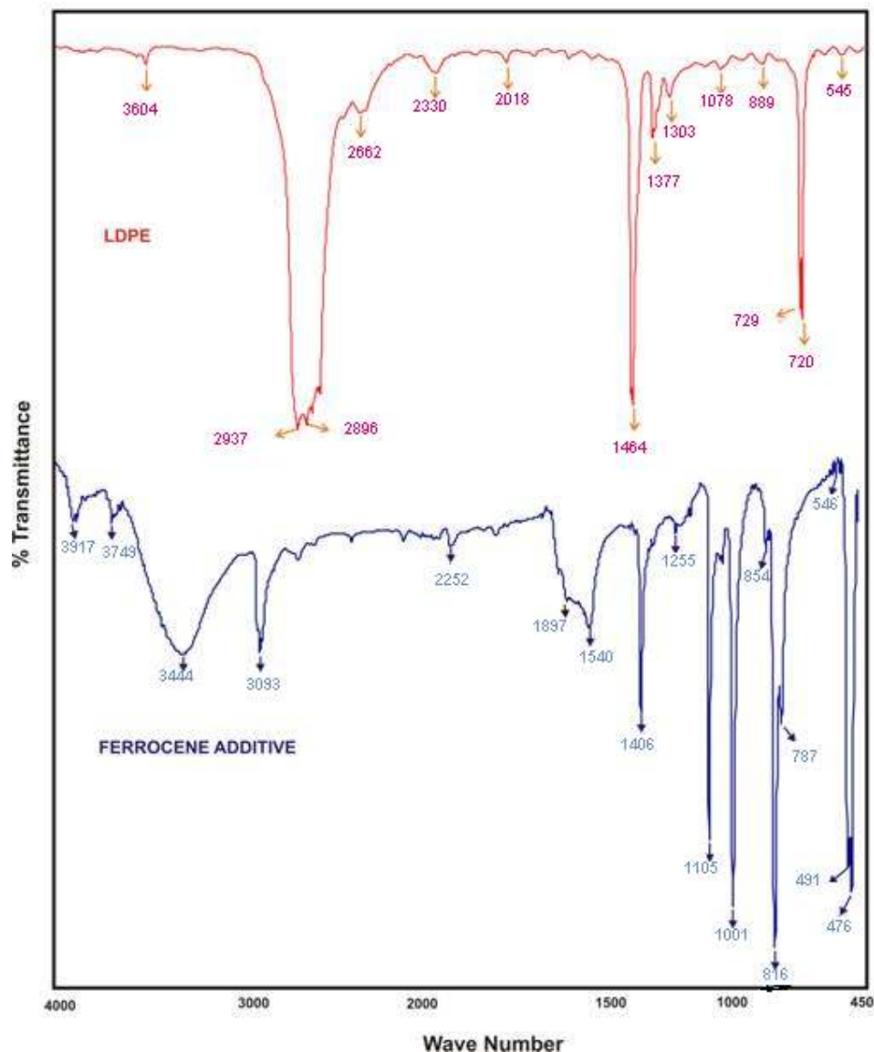
Figure.12: FTIR spectra for LDPE-Ferrocene before exposure to UV radiation
