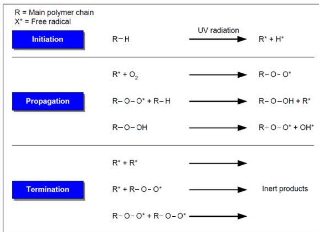
55 Figure 1: The general mechanism for photodegradation and thermal degradation
