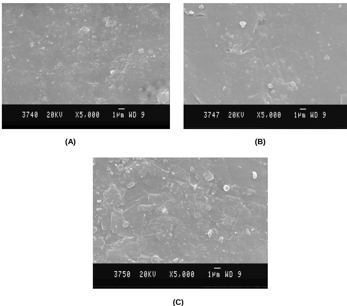
Figure. 18: (A) LDPE-Ferrocene-1% After UV exposure (B) LDPE-Ferrocene -2% After UV exposure (C) LDPE-Ferrocene-3% After UV exposure
