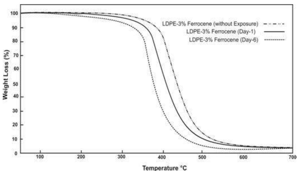
Figure.11: TGA thermogram for LDPE-3% Ferrocene after UV exposure 1 to 6 days
