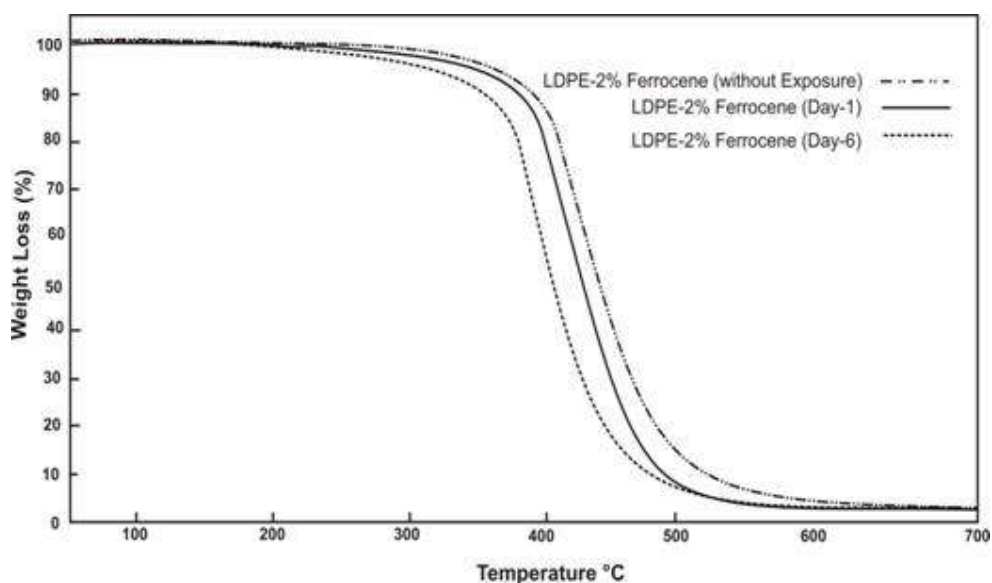
Figure.10: TGA thermogram for LDPE-2% Ferrocene after UV exposure 1 to 6 days
