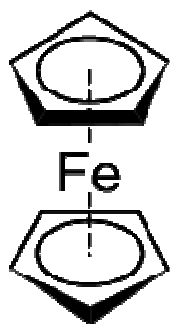
Figure. 2: Structural Formula of Ferrocene
