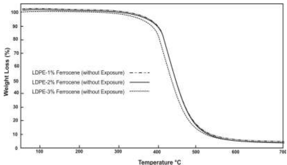
Figure. 8: TGA thermogram for LDPE-Ferrocene 1 to 3% before UV exposure
