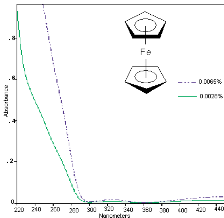
Figure. 3: UV absorption spectra for Ferrocene
