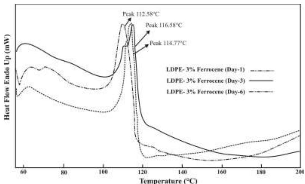
Figure.7: DSC thermo gram for LDPE-3 % Ferrocene after exposure to UV radiation
