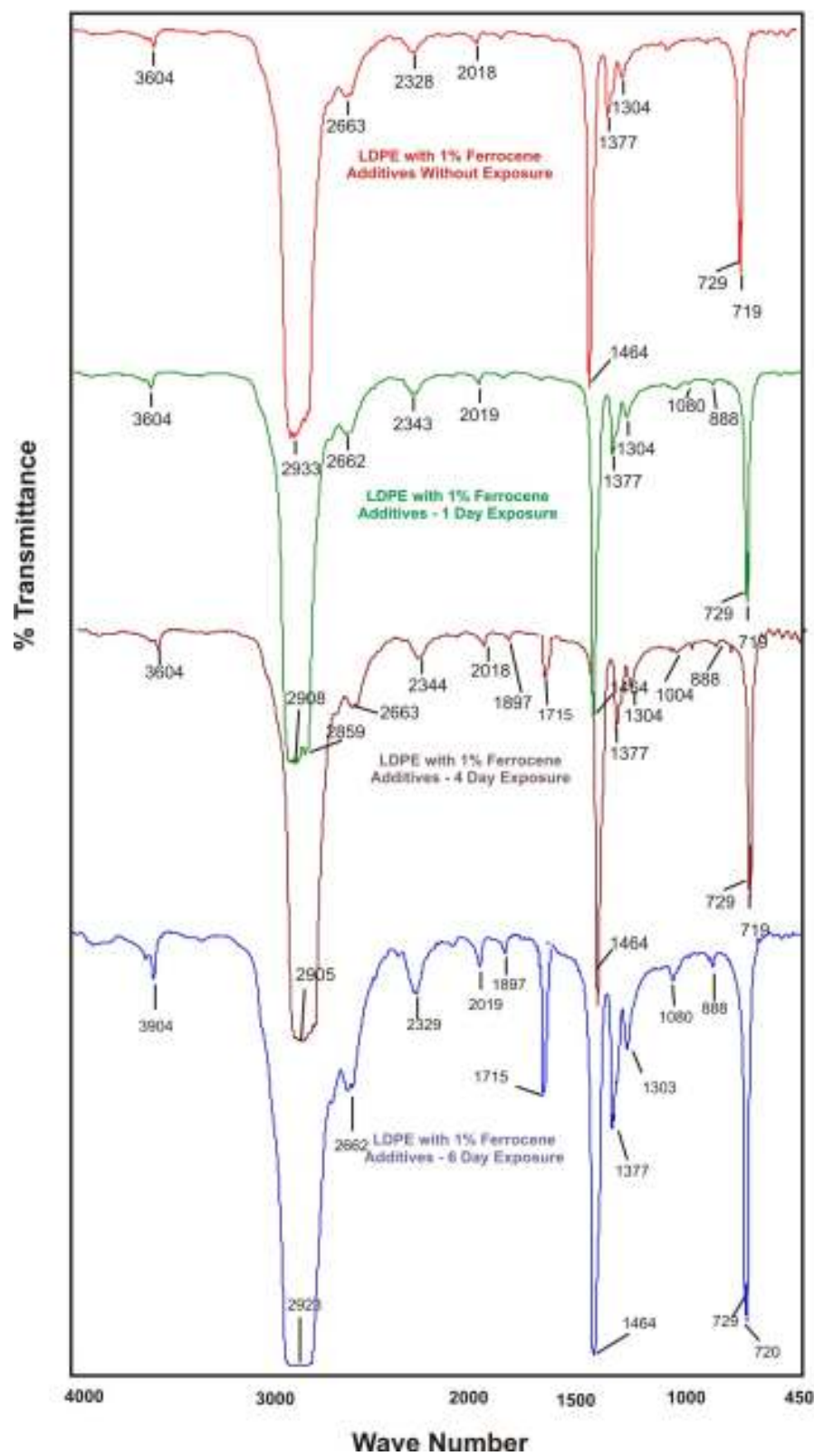
Figure. 14: FTIR spectra for LDPE-1% Ferrocene after exposure to UV radiation
