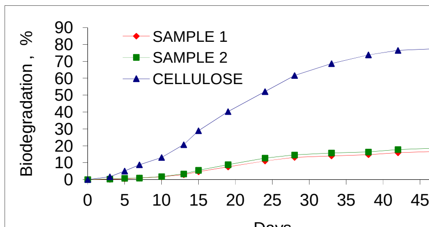
Figure.19: Bio-degradation curve for the photodegradable product of LDPE- 1% Ferrocene film
