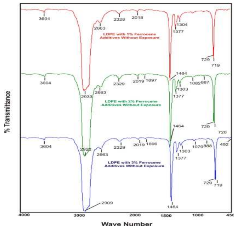
Figure.13: FTIR spectra for LDPE-1% Ferrocene, LDPE-2% Ferrocene and LDPE-3% Ferrocene before exposure to UV radiation
