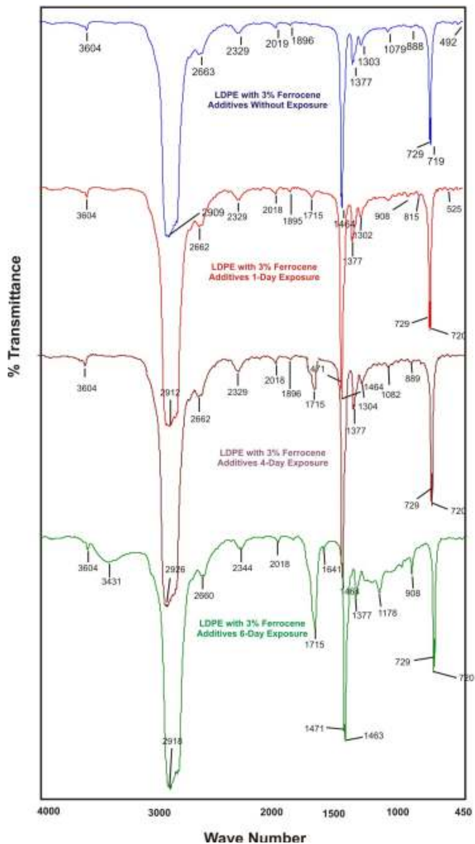
Figure.16: FTIR spectra for LDPE-3% Ferrocene after exposure to UV radiation
