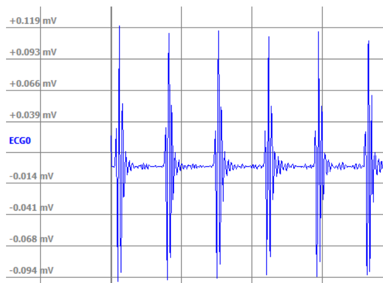
Figure 9: Record n01 after BPF between 20-30Hz
