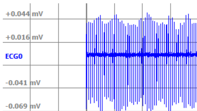
Figure 11: Record n01 after BPF at 30-50Hz
