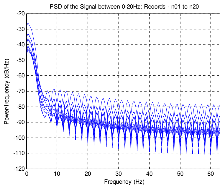
Figure 19: PSD of Even Records from n01-n20
