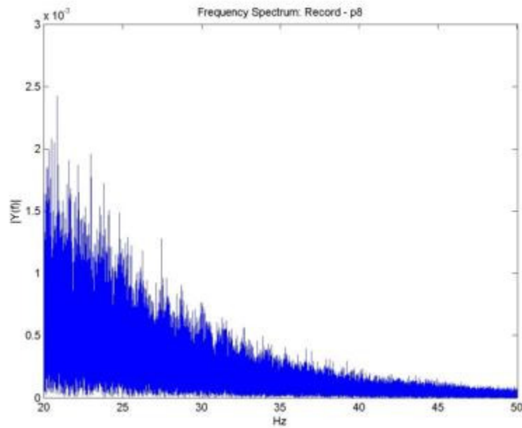
Figure 13: Spectrum(20-50Hz) of Record p08
