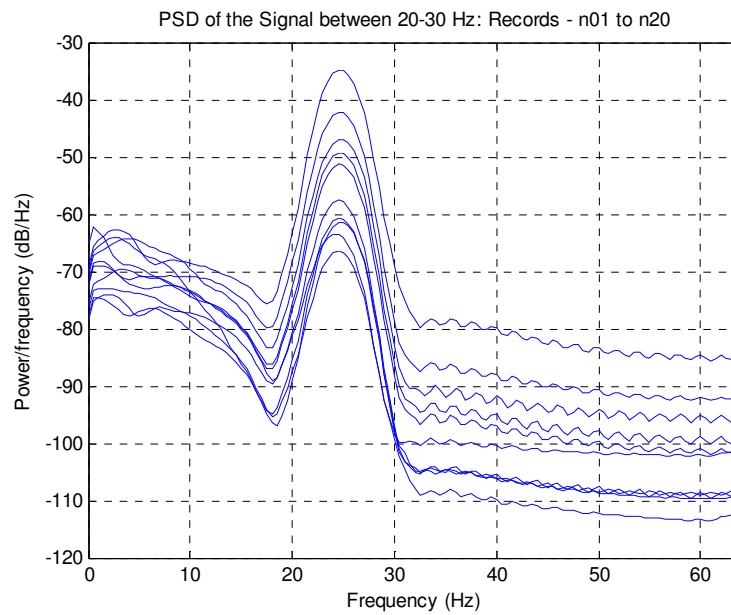
Figure 17: PSD of Even Records from n01-n20
