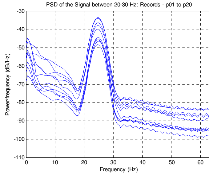
Figure 16: PSD of Even Records from p01-p20
