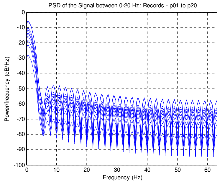
Figure 18: PSD of Even Records from n01-n20
