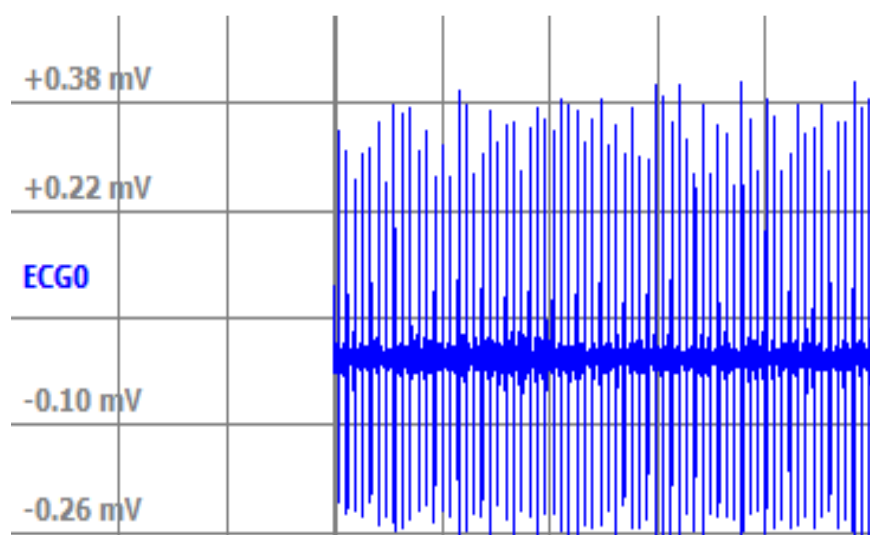
Figure 10: Record p02 after BPF at 30-50Hz
