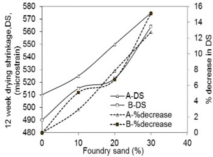
Fig. 6: Influence of foundry sand content on 12-week drying shrinkage
