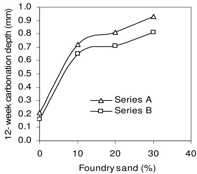
Fig. 7: Variation of carbonation depth
