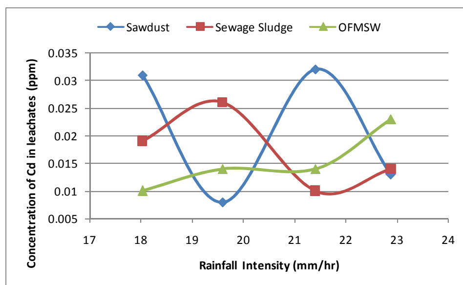
Figure 7: Concentration of Cd in leachates versus rainfall intensity
