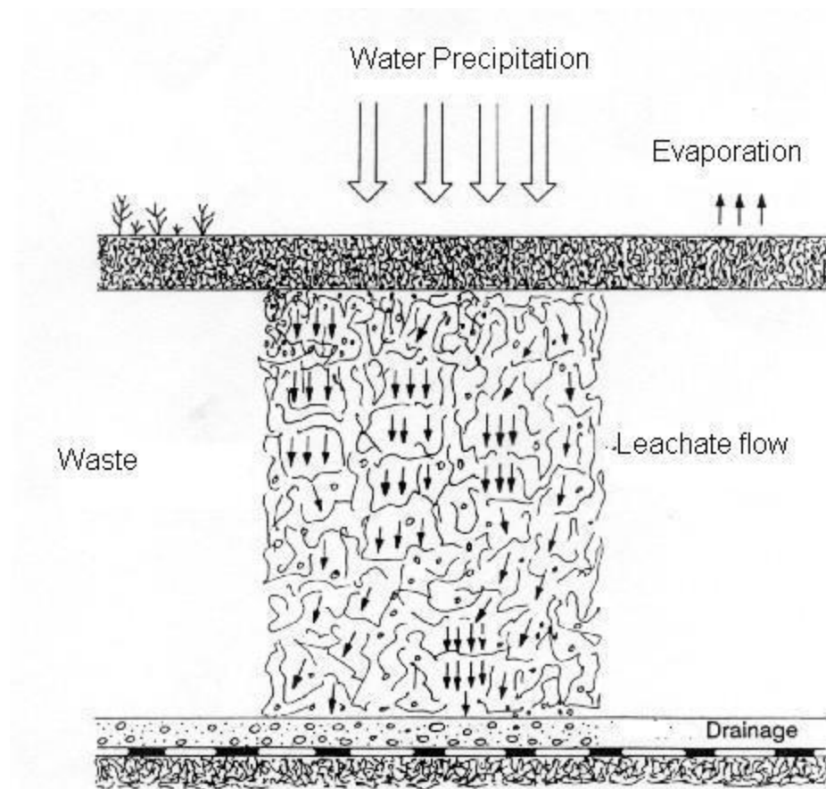
Figure 1: Schematic of leachate flow through waste
