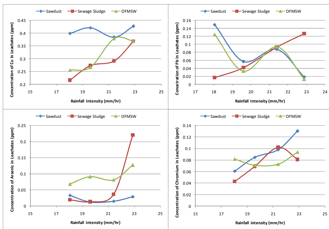
296 Figure 6: Concentration of Cu, Pb, As and Cr in leachates versus rainfall intensity
