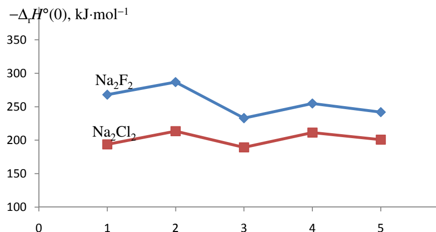
113 Figure 2. Enthalpies of dimerization reactions 2\text{NaX} = \text{Na}_2\text{X}_2 , \Delta_r H^\circ(0) versus the level of calculations: 114 1 – B3P86 MC, 2 – MP2 MC, 3 – B3P86 Ext, 4 – MP2 Ext, 5 – the reference from 115 IVTANTHERMODatabase [14].
