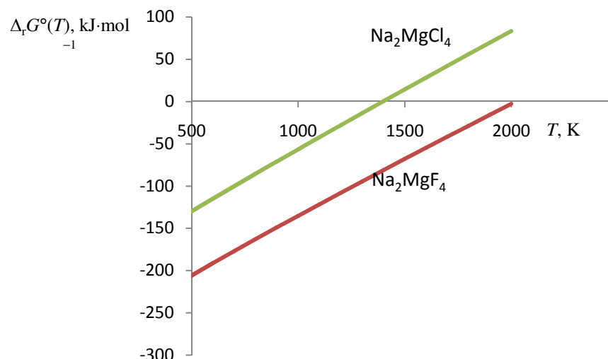
Figure 7. Gibbs free energy change against temperature for reaction \text{Na}_2\text{X}_2 + \text{MgX}_2 = \text{Na}_2\text{MgX}_4 ; the polyhedral isomer ( C_{2v} ) for \text{Na}_2\text{MgX}_4 was considered
