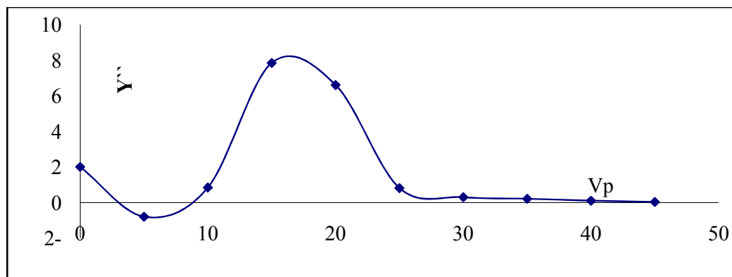
Figure8(a) The second derivative of the electron current for cathode fall
