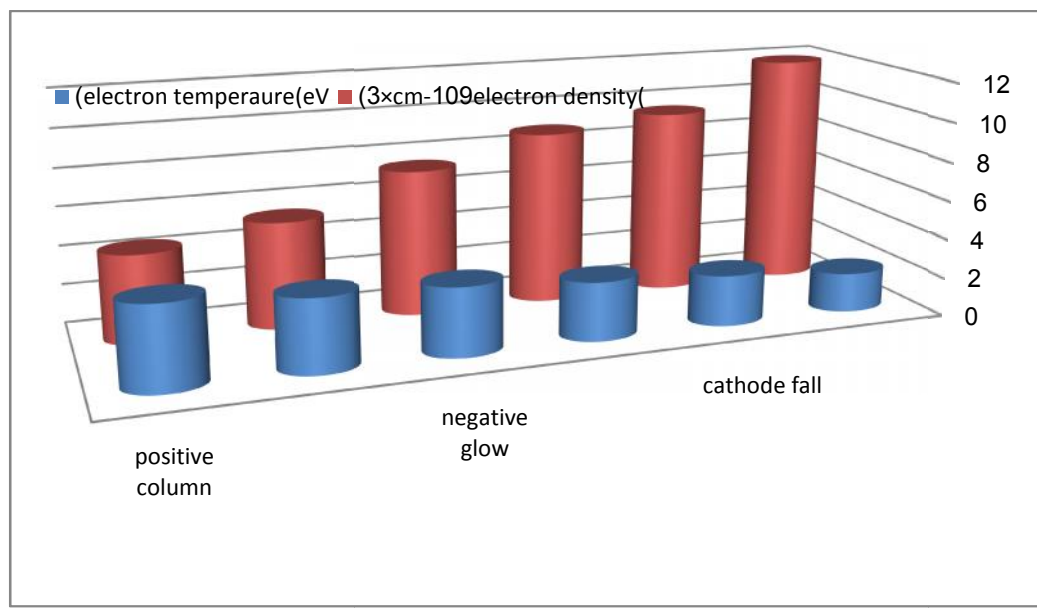
Figure (11) axial electron temperature and density distributions at edge in the presence of magnetic field.
