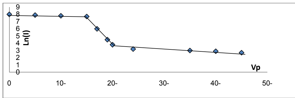
Figure7(b) Semi-Log curve of the electron current for negative glow region.
