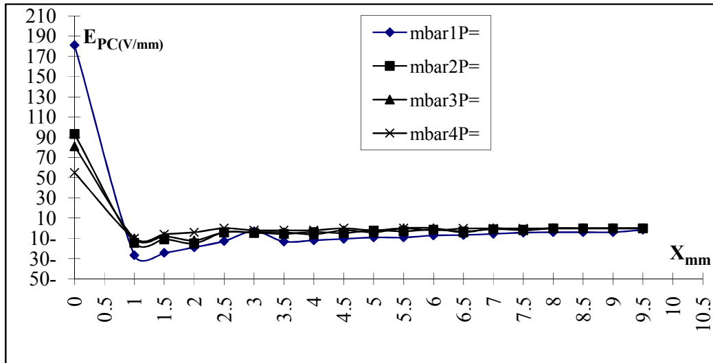
Figure(4) Axial electric field distribution in at edge in the Presence of magnetic field at constant current( I=10\text{mA} )
