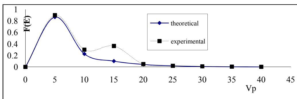
Figure 10(b ) Comparison between the experimental and theortical of EEDF for negative glow
