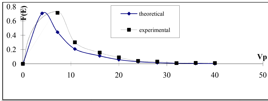
Figure10(c) Comparison between the experimental and theortical of EEDF for Positive column
