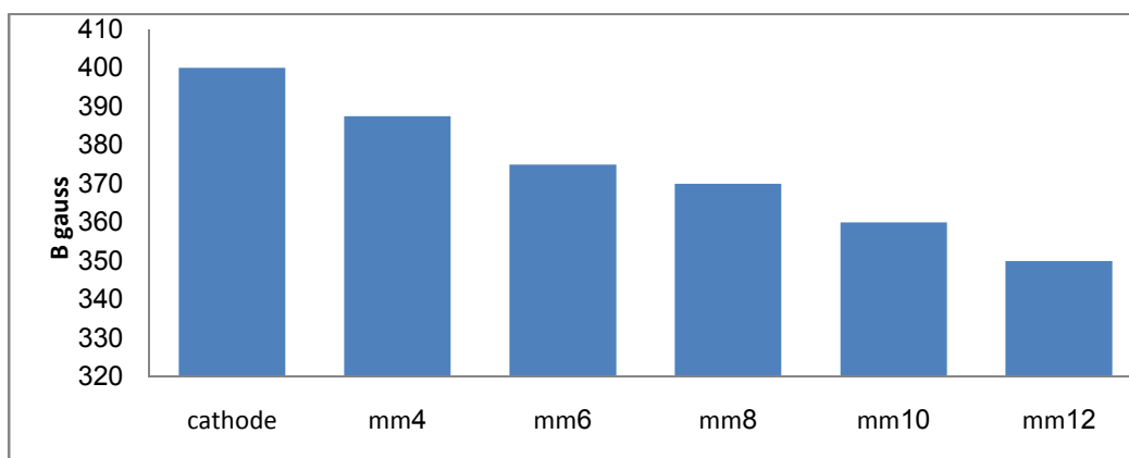
Figure (2) axial distribution of the magnetic field strength
