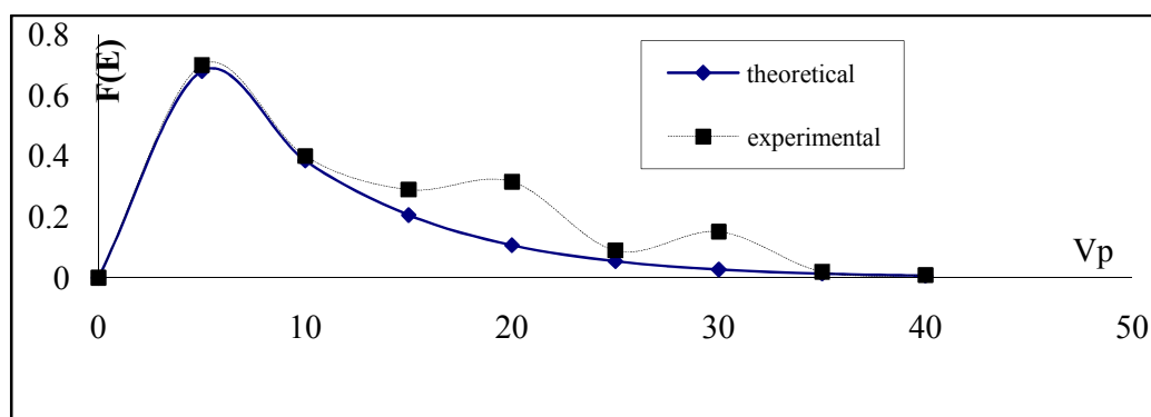
Figure 10(a ) Comparison between the experimental and theortical of EEDF for cathode fall
