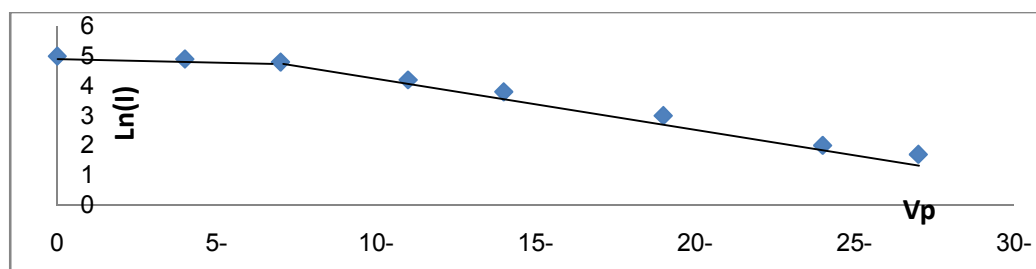
Figure7(c) Semi-Log curve of the electron current for Positive column region.
