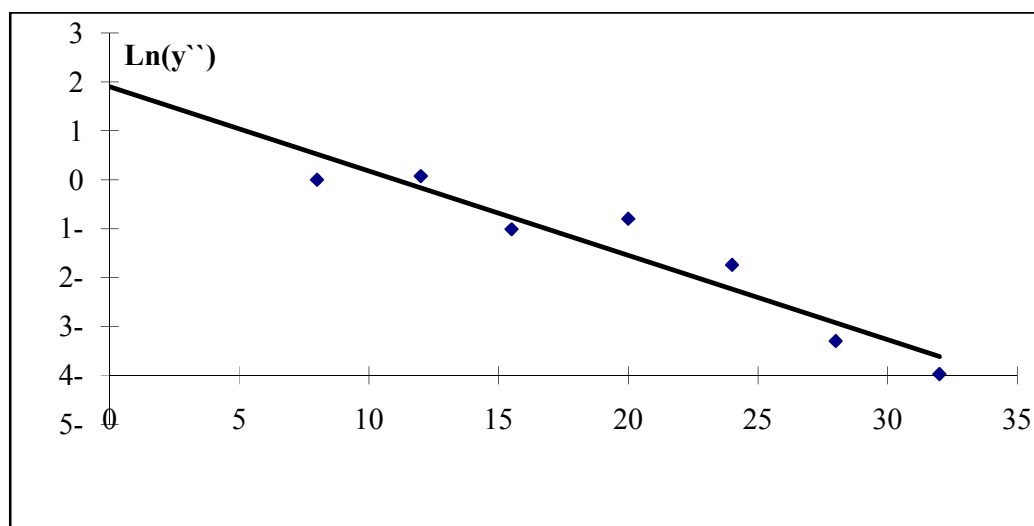
Figure9(c) Semi- Log of the second derivative of the electron current for positive column
