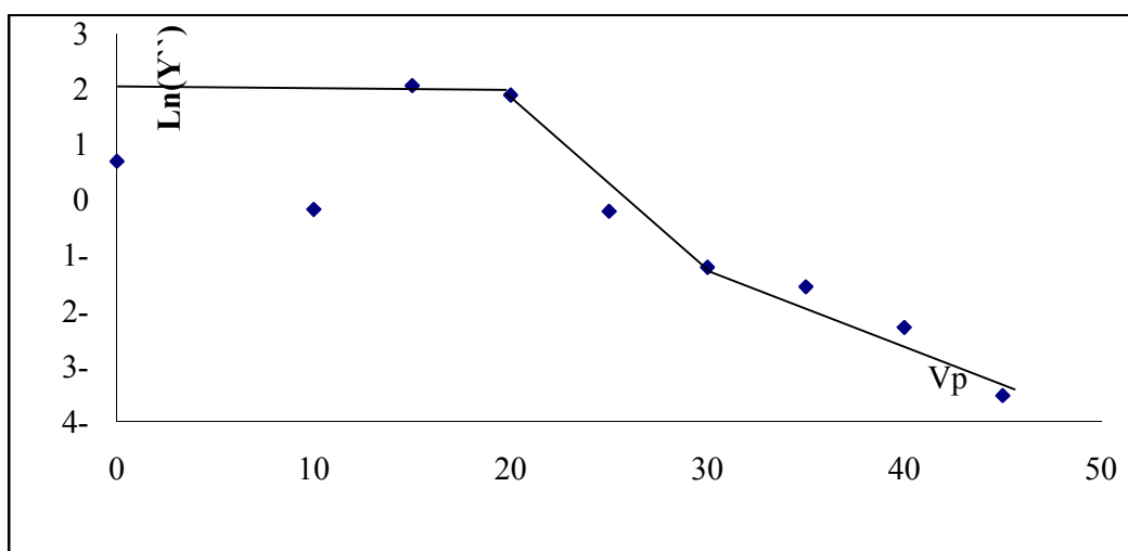
Figure 9(a ) Semi-Log curve of The second derivative of the electron current for cathode fall
