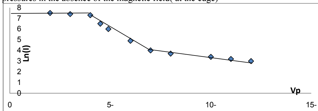
Figure 7(a) Semi-Log curve of the electron current for cathode fall region
