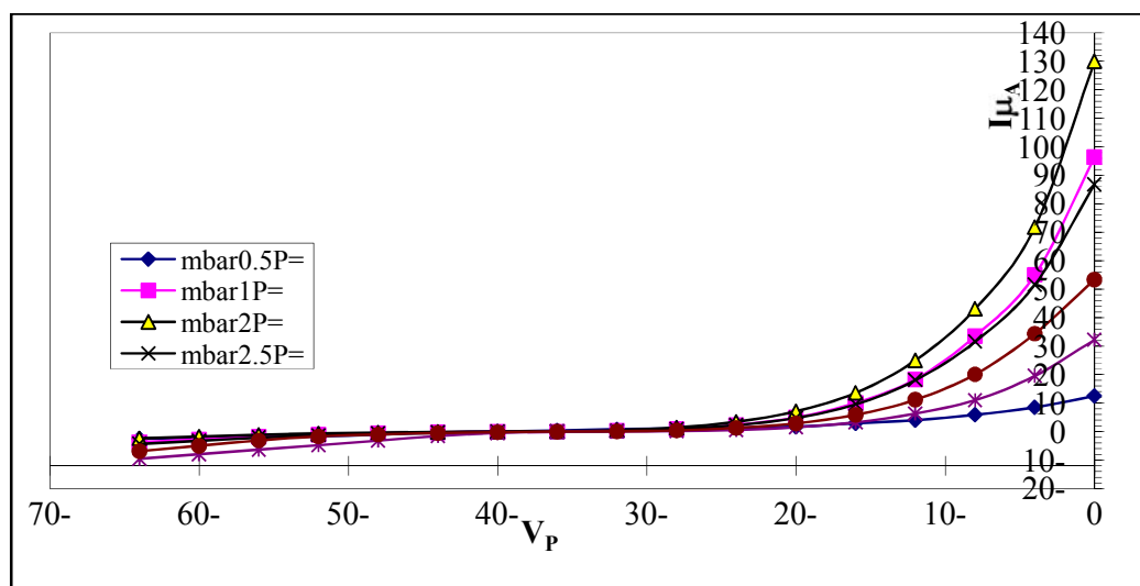
Figure(5) I-V curves of the single probe for cathode fall region at different Ar pressures in the absence of the magnetic field( at the edge)
