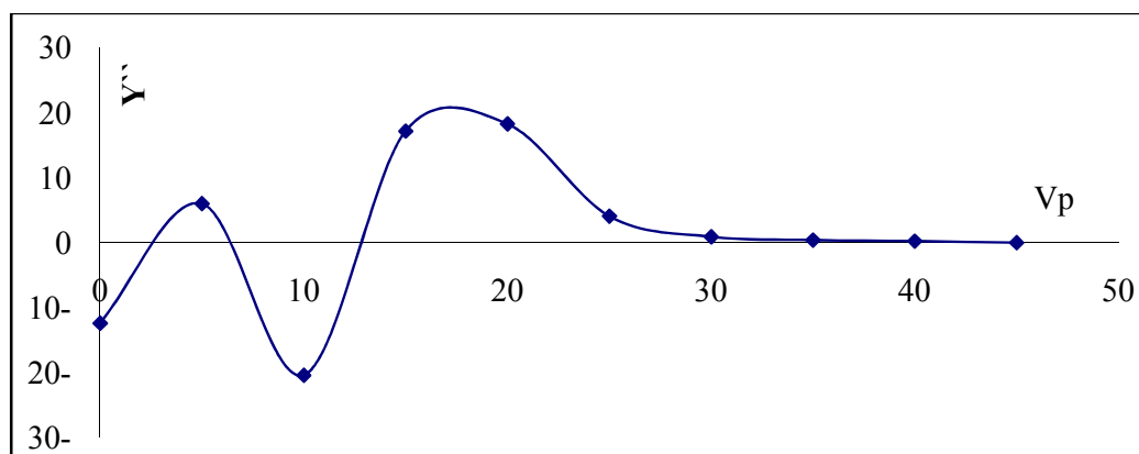
Figure8(b) The second derivative of the electron current for negative glow
