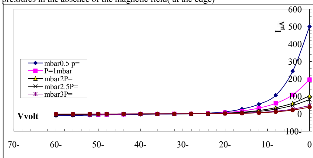
Figure(6) I-V curves of the single probe for cathode fall region at different Ar pressures in the absence of the magnetic field( at the edge)
