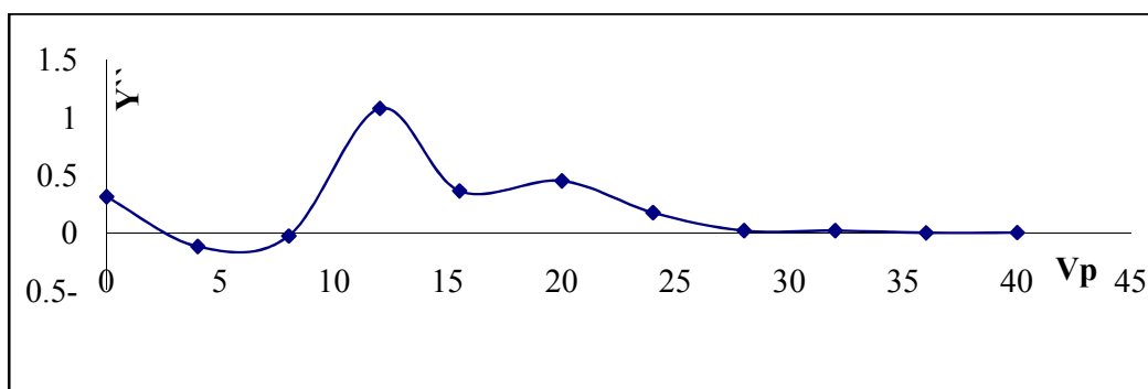
Figure8(c) The second derivative of the electron current for Postive column
