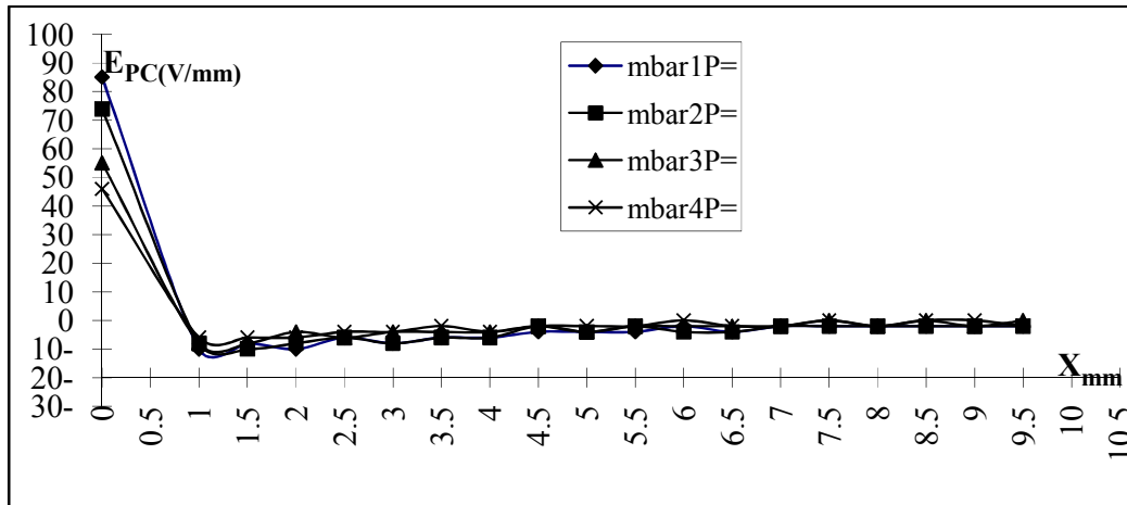
Figure(3) Axial electric field distribution in at edge in the absence of magnetic field at constant current( I=10\text{mA} )
