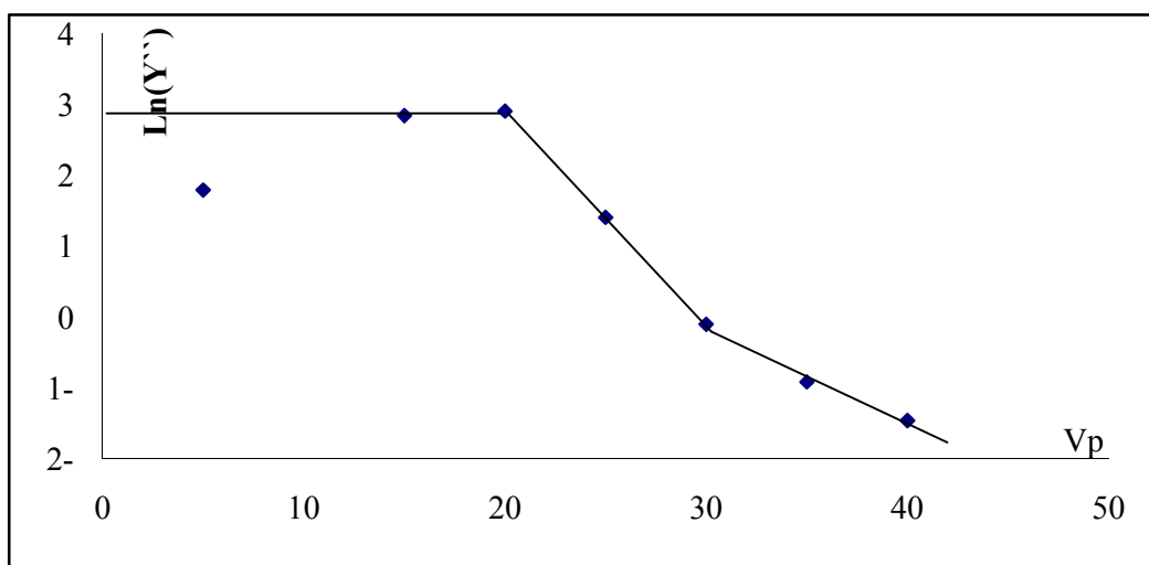
Figure 9(b) Semi- Log of the second derivative of the electron current for negative glow
