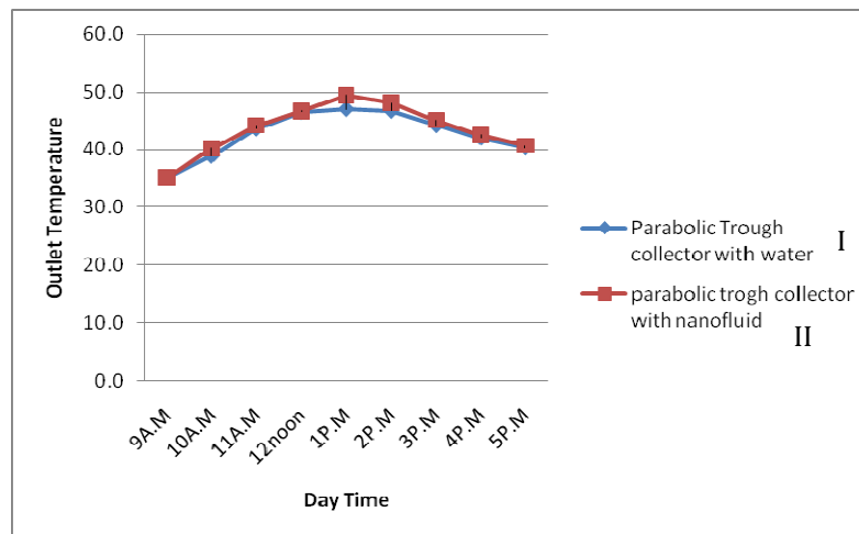
128 Fig 4:- Hot water outlet temperature Vs Day time as per various test set ups. 129 (Full sun shine day)
