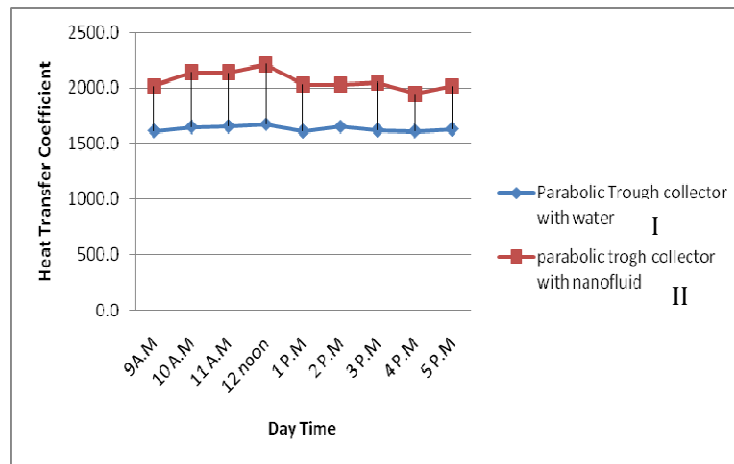
Fig 6: - Heat transfer coefficient Vs Day time as per various test set up. (Full sun shine day).
