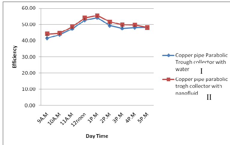
Fig 5: - Solar thermal efficiency Vs day time as per various test set ups. (Full sun shine day)
