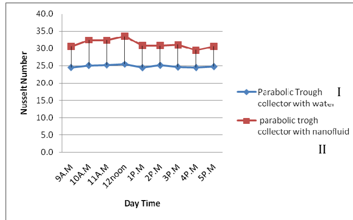
Fig. 7: - Nusselt number Vs Day time as per various test of set up. (Full sun shine day).
