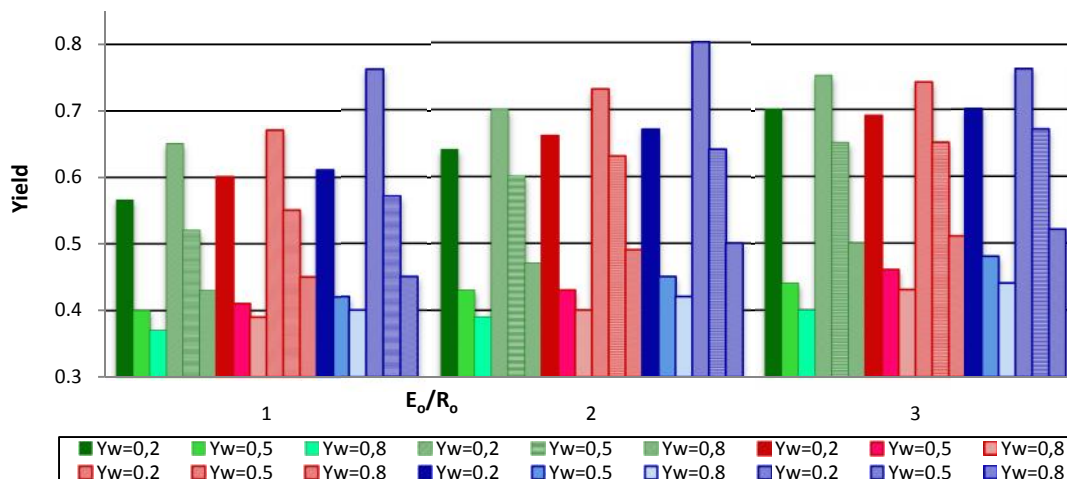
Fig.7. The Effect of Mole Fraction of Water in Solvent ( Y_w ) and Mole Fraction Ratio of Solvent to Feed ( E_o/R_o ) for the Yield of Phenol (green), o-Cresol (red), and p-Cresol (blue) at 308 K with Acetone Solution (solid) and Methanol Solution (pattern)
