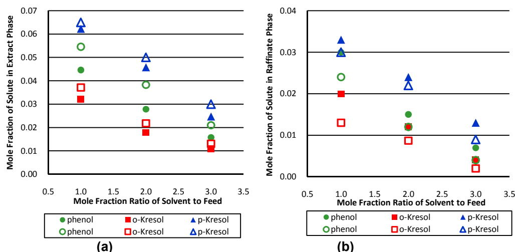
Fig. 1. The Effect of Mole Fraction Ratio of Solvent to Feed for Mole Fraction of Phenol, o -Cresol, and p -Cresol in Extract Phase (a) and Raffinate Phase (b) at 308 K and Y_w=0.2 with Acetone Solution (black) and Methanol Solution (white)
