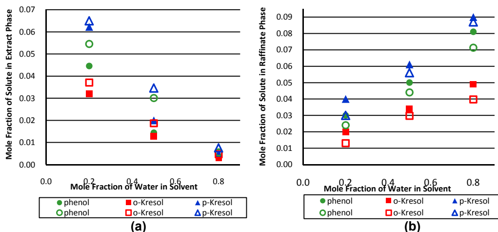
Fig.3.The Effect of Mole Fraction of Water in Solvent for the Mole Fraction of Phenol, o-Cresol, and p-Cresol in Extract Phase (a) and Raffinate Phase (b) at E_0/R_0=1 dan T = 308 K with Acetone Solution (black) and Methanol Solution (white)
