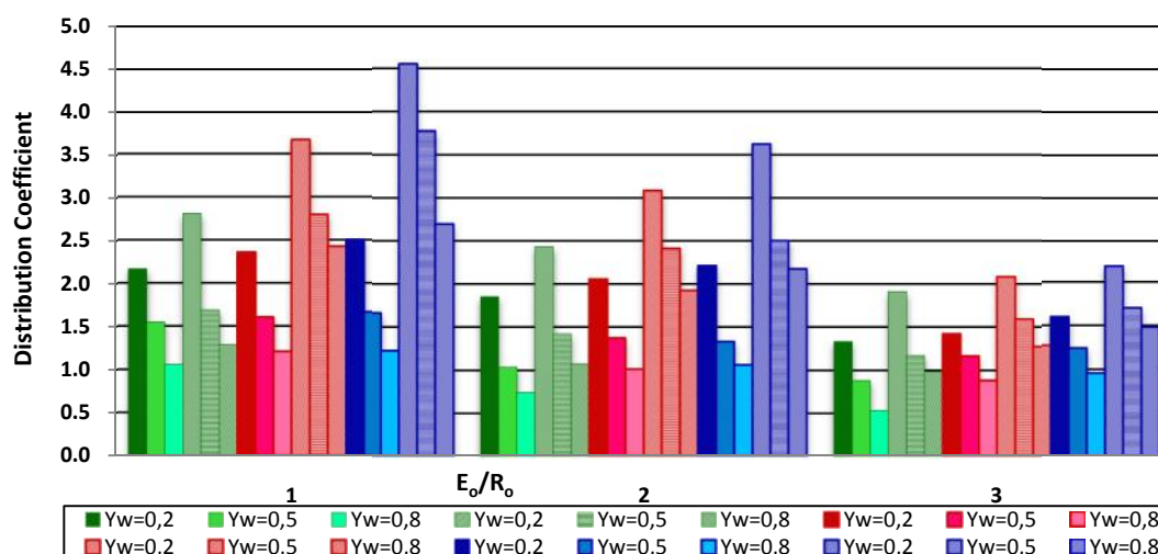
Fig.5.The Effect of Mole Fraction of Water in Solvent ( Y_w ) and Mole Fraction Ratio of Solvent to Feed ( E_o/R_o ) for the Distribution Coefficient of Phenol (green), o-Cresol (red), and p-Cresol (blue) at 308 K with Acetone Solution (solid) and Methanol Solution (pattern)
