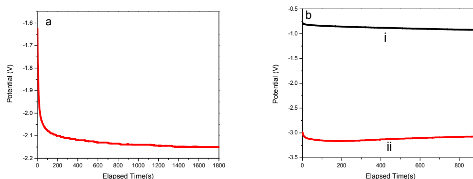
Fig. 1a) Galvenostatic reduction of GO in 0.5 M \text{H}_2\text{SO}_4 at 1 \text{ mA/cm}^2 . b) Galvenostatic deposition of Pt from chloro platonic acid at 2 \text{ mA/cm}^2 onto i) rGO/C-felt ii) rGO/C-felt and C-felt in series.
