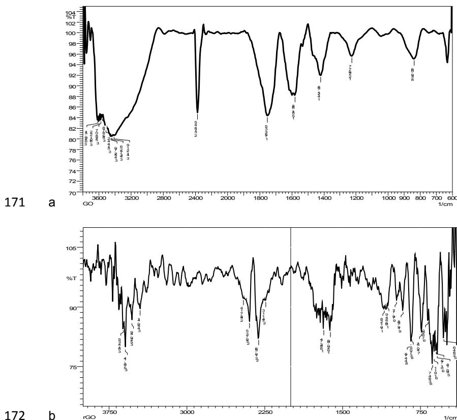
Fig. 2. FT-IR spectra of a) Graphene Oxide (GO) b) Reduced Graphene Oxide (rGO).
