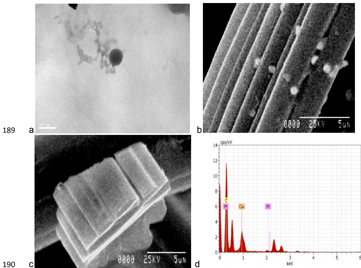
Fig. 3. TEM image of a) Pt nano particles onto rGO surface b) SEM image of Pt nano particles onto rGO/C-felt surface c) SEM image of exfoliated rGO onto C-felt surface d) EDX spectra of Pt/rGO composite.
