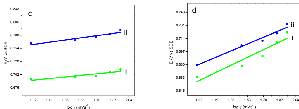
Fig. 6. (a) (b) I_{pc} vs \sqrt{v} and (c) (d) E_{pc} vs \log v plots of i) Pt/rGO/C-felt and ii) Pt/C-felt at different scan rates (10, 30, 50, 70 and 90 mV/s) for MeOH (a, c) and EtOH (b, d).
