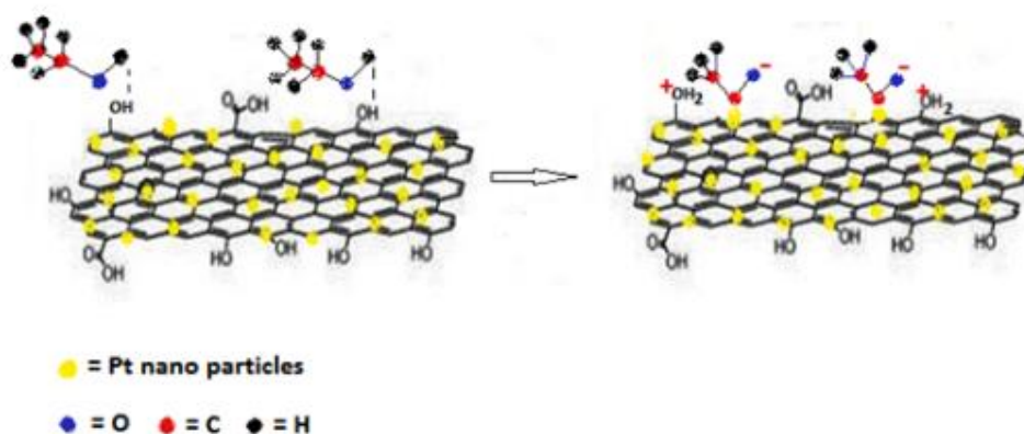
306 Fig. 8. Proposed model indicating attachment of EtOH on to Pt/rGO/C-felt surface followed by 307 its H-bond assisted deprotonation. 308
