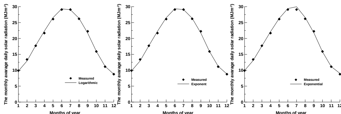
Figure 3. Comparison of empirical models with measured values.
