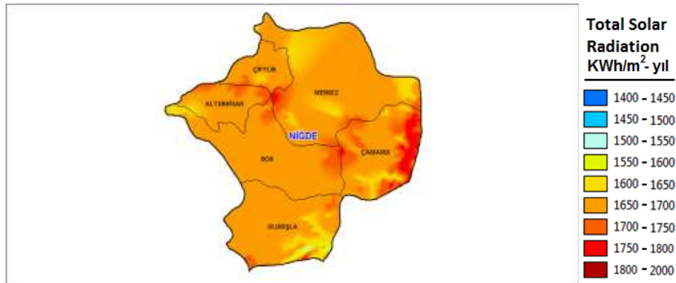
Figure 2. Solar Map of Nigde, Turkey
