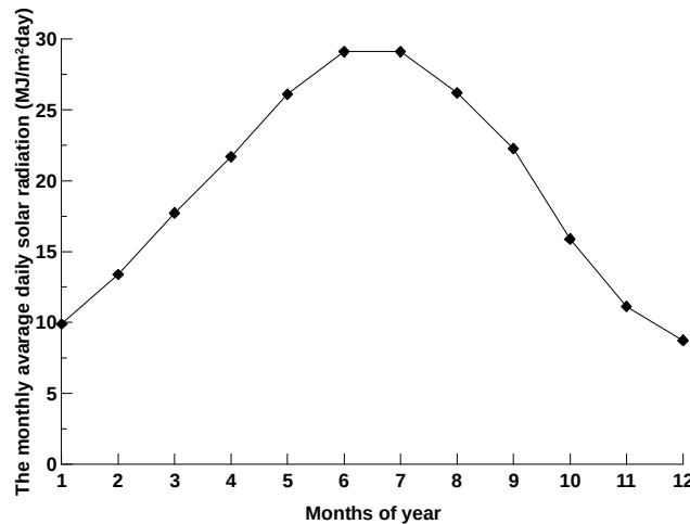
Figure 1. The measured monthly mean daily global solar radiation in Nigde.
