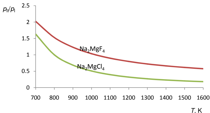
Figure 5. Relative abundance p_{II}/p_I of two isomers of supersalts \text{Na}_2\text{MgF}_4 and \text{Na}_2\text{MgCl}_4 ; I is D_{2d} and II is C_{2v} isomer (MP2 Ext)
