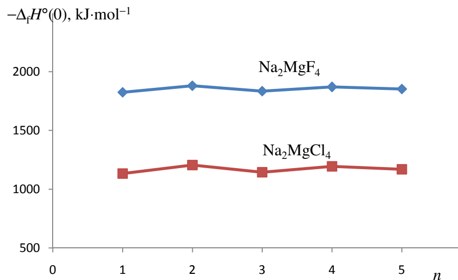
Figure 6. The enthalpies of formation of the salts calculated through different approaches: n = 1, 2 correspond to reaction 2\text{NaX} + \text{MgX}_2 = \text{Na}_2\text{MgX}_4 (1 – B3P86 EXT, 2 – MP2 EXT); n = 3, 4 correspond to reaction \text{Na}_2\text{X}_2 + \text{MgX}_2 = \text{Na}_2\text{MgX}_4 (3 – B3P86 EXT, 4 – MP2 EXT); n = 5 correspond to the averaged values
