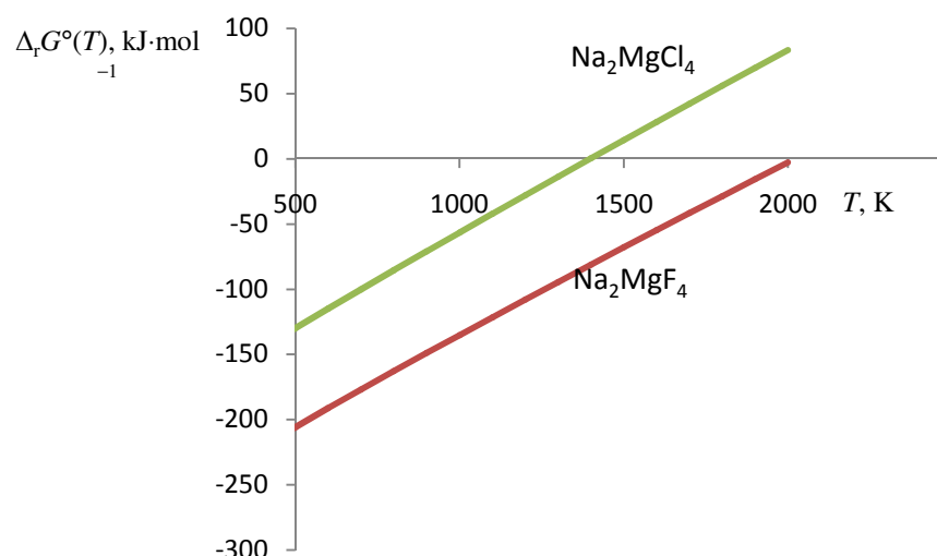
Figure 7. Gibbs free energy change against temperature for reaction \text{Na}_2\text{X}_2 + \text{MgX}_2 = \text{Na}_2\text{MgX}_4 ; the polyhedral isomer ( C_{2v} ) for \text{Na}_2\text{MgX}_4 was considered
