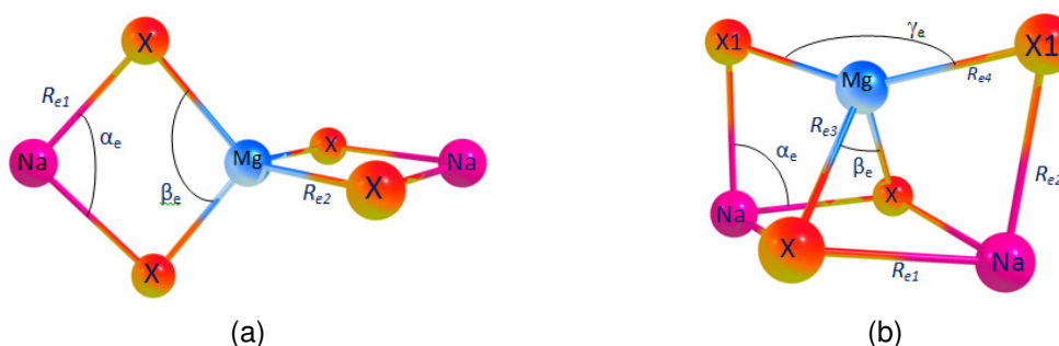
Figure 3. Equilibrium geometrical configurations of Na_2MgX_4 isomers: (a) two-cycled structure of D_{2d} symmetry; (b) polyhedral structure of C_{2v} symmetry
