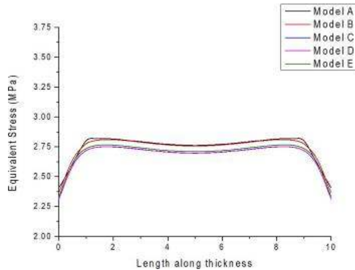
Fig. 2.2 Plot of equivalent stress along the thickness of the disc
