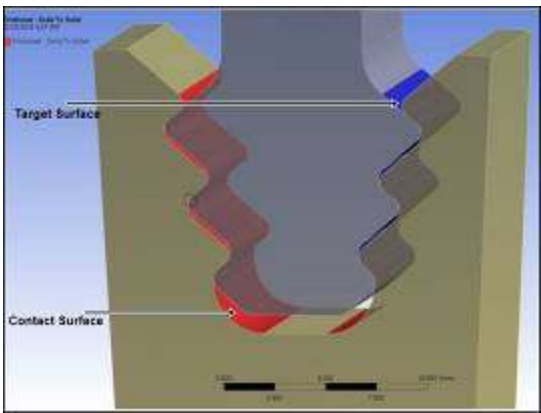
Figure 2.4: Contact and target faces at the blade disc interface
