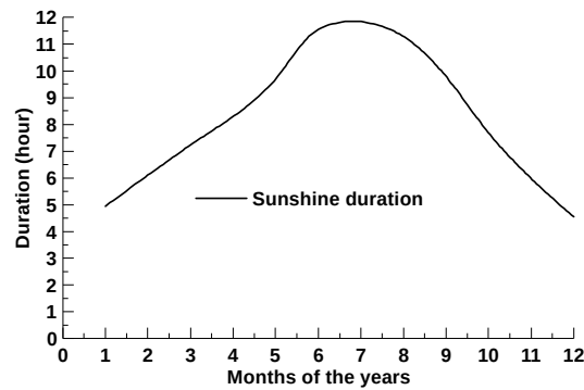
Fig. 2 Sunshine duration throughout the year
