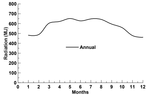
Fig 7. Annually average solar radiation availability of tilted surfaces.
