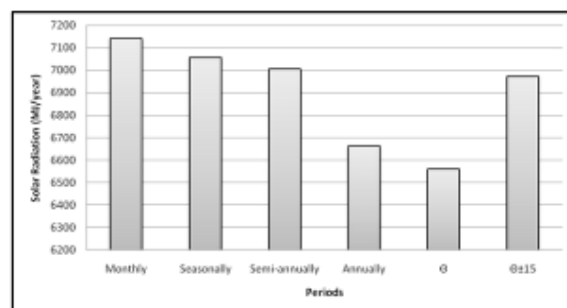
Fig 4. Solar radiations on tilted surface for optimum tilt angles
