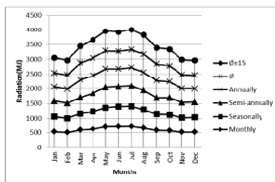
Fig 3. Monthly, seasonally, semi-annually, annually, latitude \pm 15 and latitude optimum tilt angles
