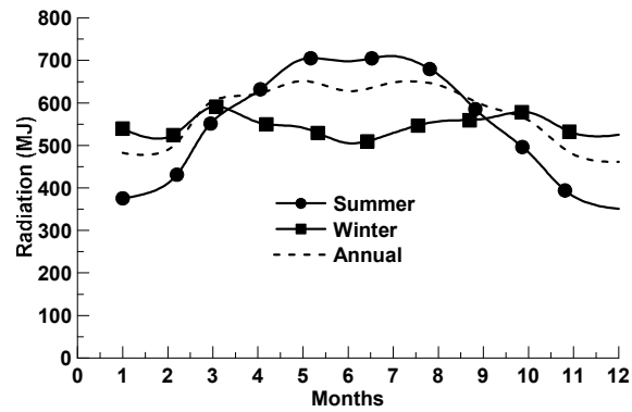
Fig 6. Semi-annually average solar radiation availability of tilted surfaces.
