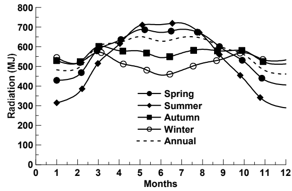
Fig 5. Seasonally average solar radiation availability of tilted surfaces.
