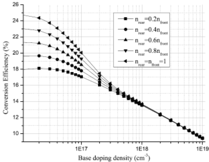
Fig. 6. Bifacial conversion efficiency versus base doping density for various rear illumination levels ( H=0.02\text{cm} , S_b = 10^3\text{cm/s} ).
