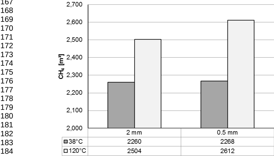
Figure 2: COD of hay with different particle sizes and temperatures
