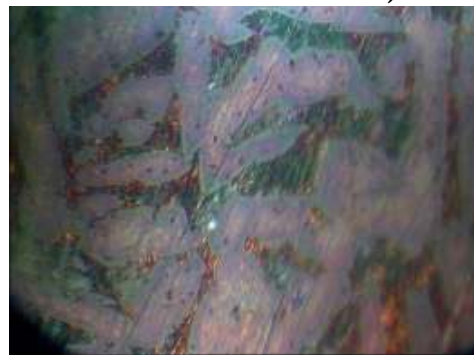
Brass+100ppm PASAC-11+S1-400x d)
