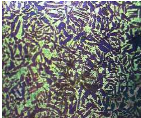
Brass+20ppm PASAC-13+S1-200x e)
