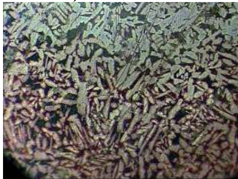
Brass+50ppm PASAC-11+S1-200x c)
