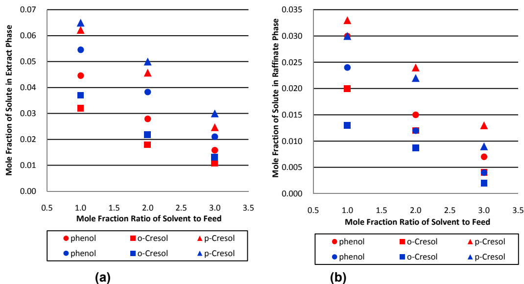
Fig. 1. The Effect of Mole Fraction Ratio of Solvent to Feed for Mole Fraction of Phenol, o-Cresol, and p-Cresol in Extract Phase (a) and Raffinate Phase (b) at 308 K and Y_w=0.2 with Acetone Solution (red) and Methanol Solution (blue)
