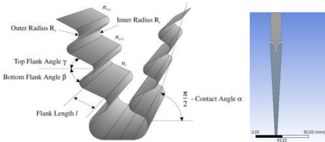
Figure 2.1 Nomenclature of fir tree root [5] and the geometrical model developed using ANSYS Workbench 14.5
