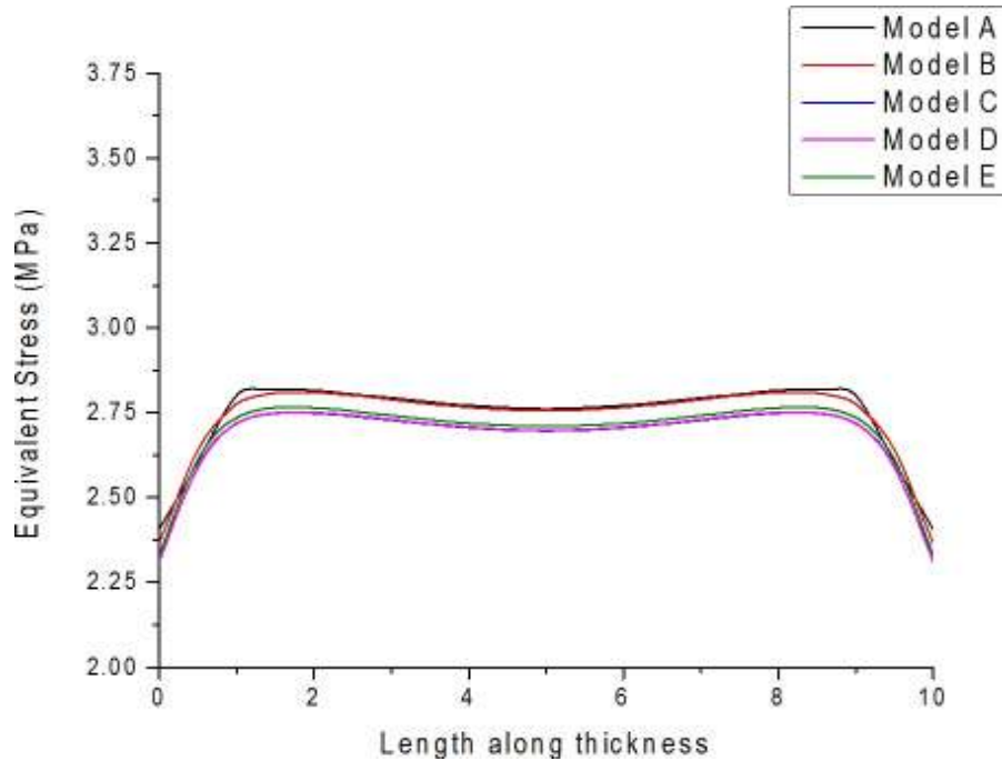
Fig. 2.2 Plot of equivalent stress along the thickness of the disc
