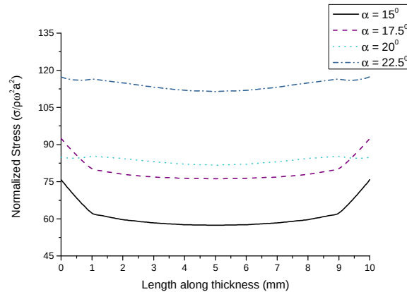
Fig 3.3 Linearized stress along the thickness for varying alpha angles
