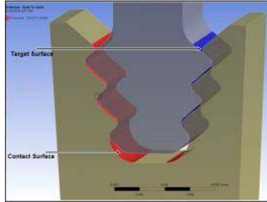
Figure 2.4: Contact and target faces at the blade disc interface
