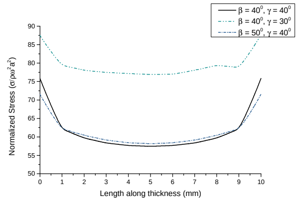
Fig 3.11 Linearized stress along the thickness for different combinations of top and bottom flank angles
