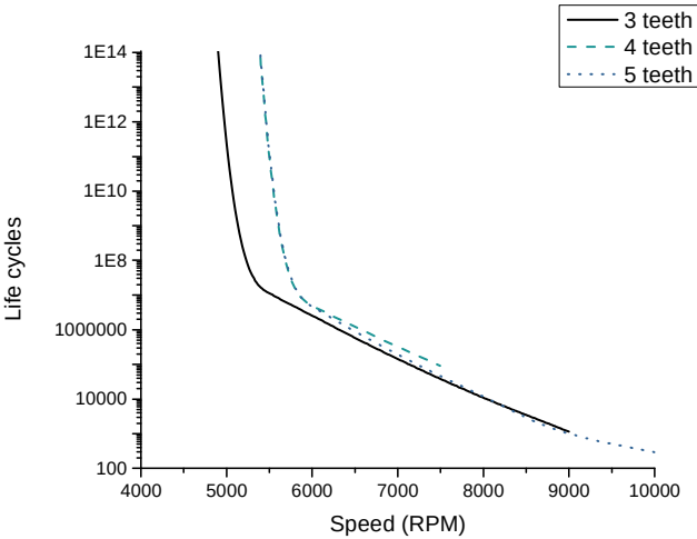
Fig 3.8 Fatigue life of the assembly vs speed for varying number of teeth
