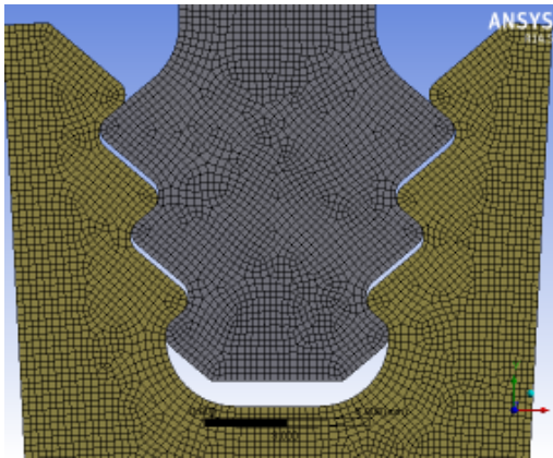
Fig 2.3(a) Uniform hex mesh of the assembly
