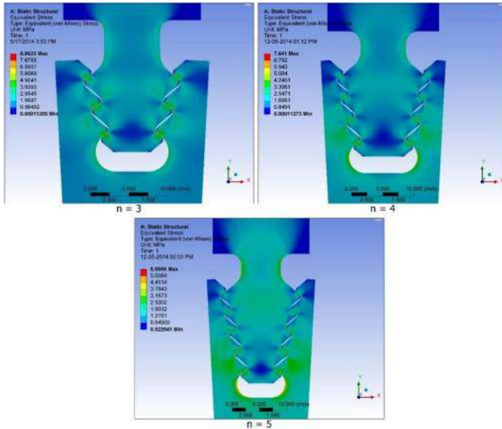
Fig 3.5 Equivalent stress contour plots for varying number of teeth
