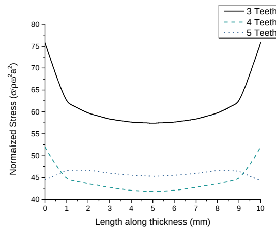
Fig 3.7 Linearized stress along the thickness for varying number of teeth
