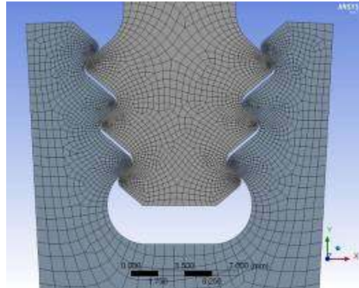
Fig 2.3(b) Hex mesh having a finer mesh at the contact faces
