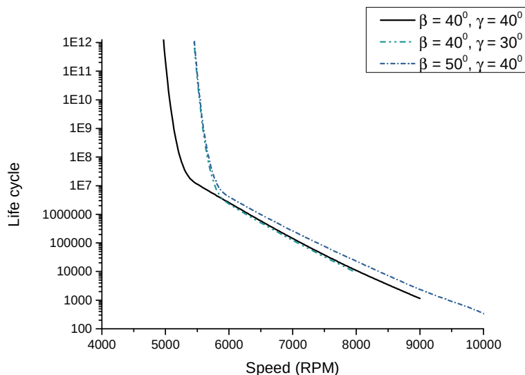
Fig 3.12 Fatigue life of the assembly vs speed for different combinations of flank angles
