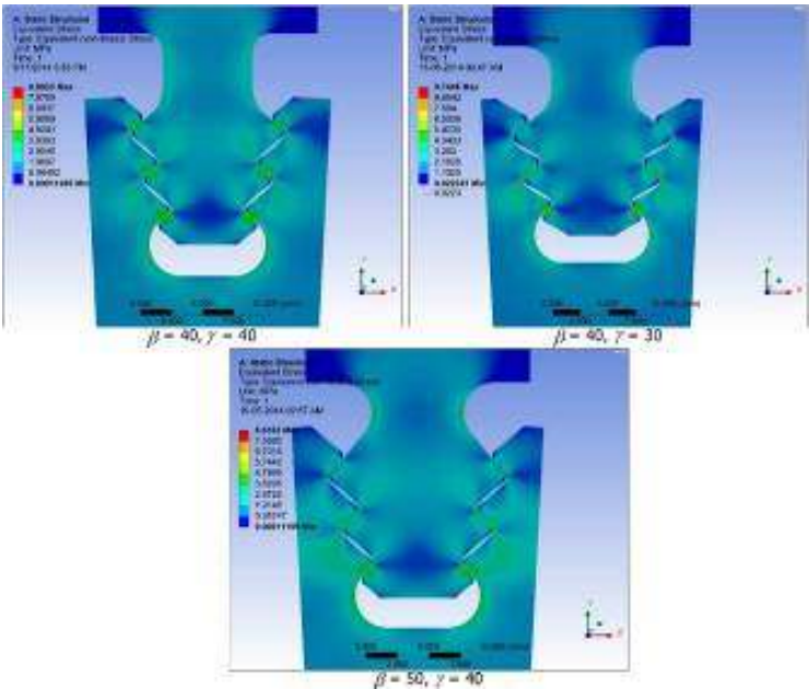
Fig 3.9 Equivalent stress contour plots for varying top and bottom flank angles
