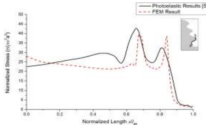
Figure 2.5 Validation graph of normalized length vs Normalized stress for photo-elastic maximum shear stress contours and Finite Element predictions.
