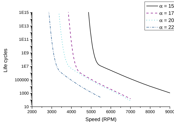
Fig 3.4 Fatigue life of the assembly vs speed for different alpha angles
