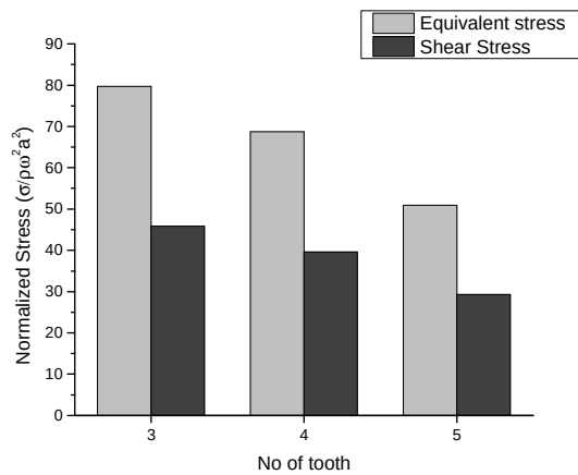
Fig 3.6 Graph of normalized Von Mises and shear stress with no of tooth ( n_i )
