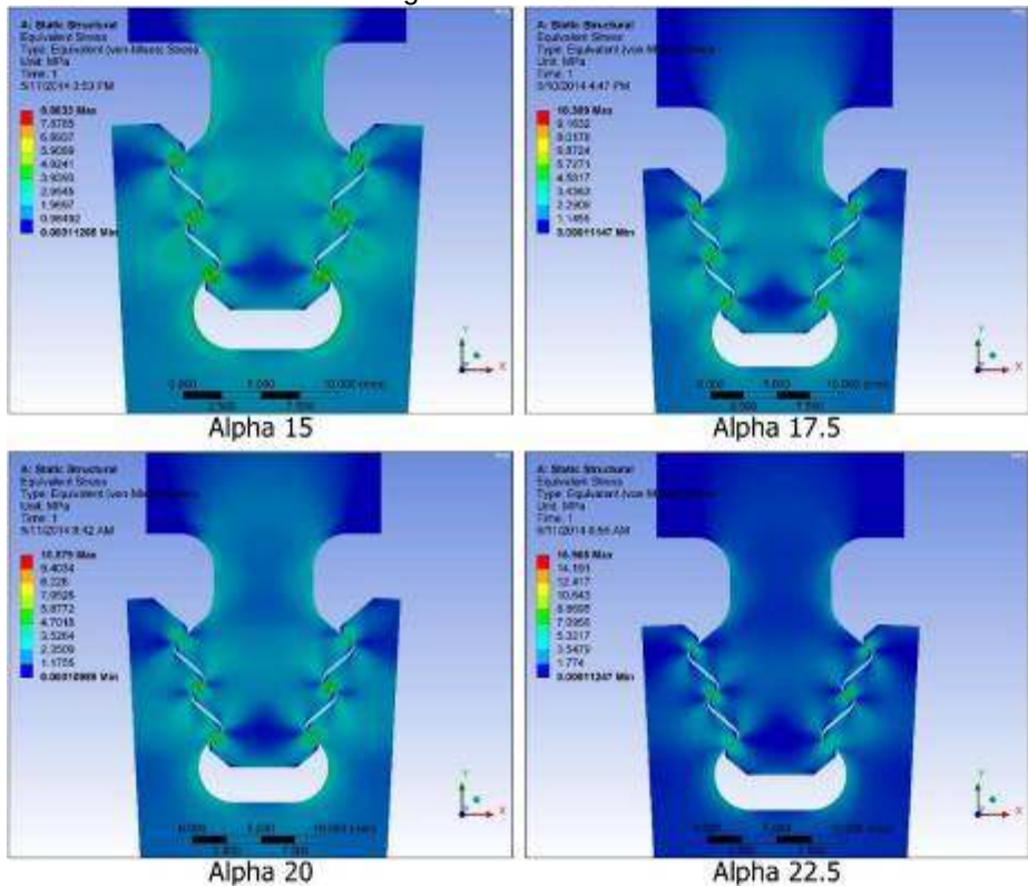
Figure 3.1 Equivalent stress contour plots of varying alpha angles
