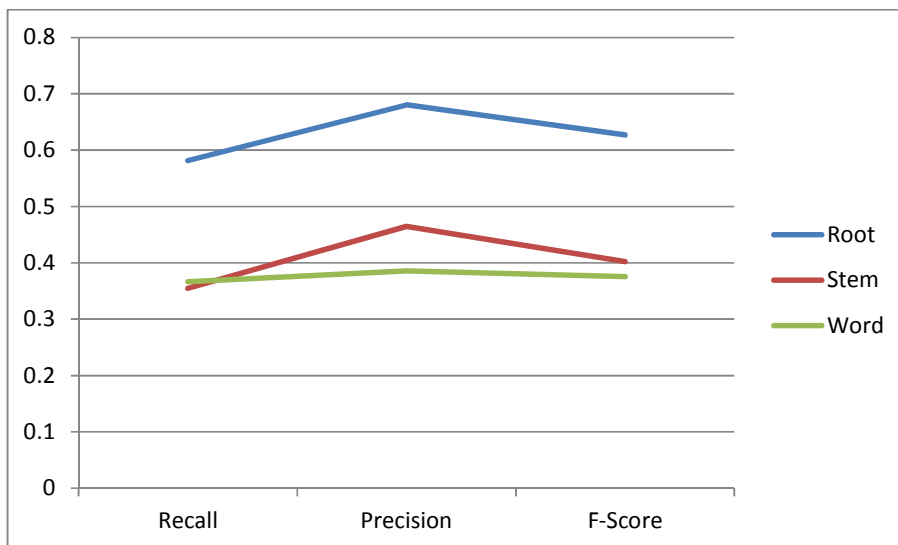
Fig.4. Comparison of Representation Models on NEWSWIRE-a Dataset
