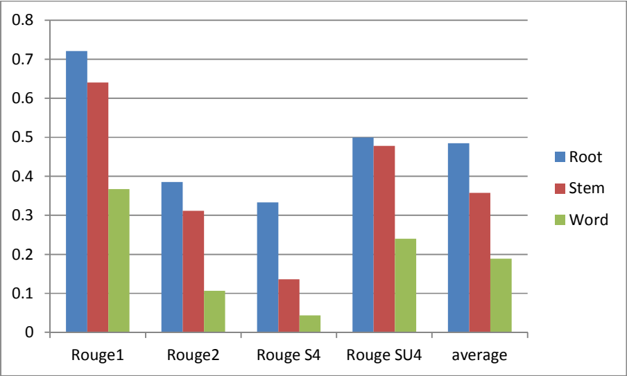
Fig.5.Rouge scores for Representative Models on NEWSWIRE-a Dataset
