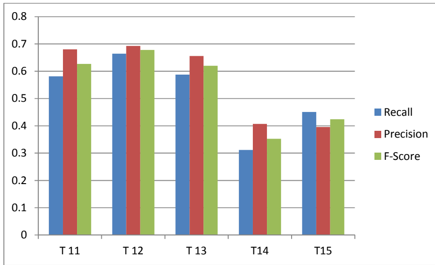
Fig.6. Comparison of Different Weighting Techniques on NEWSWIRE-a Dataset
